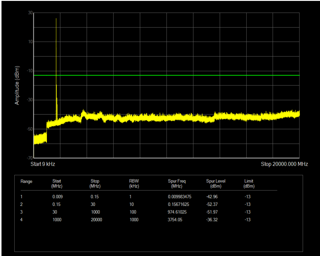
n66 SCS=15kHz DFT_QPSK BW=5MHz Channel=342500 RB=1@24
