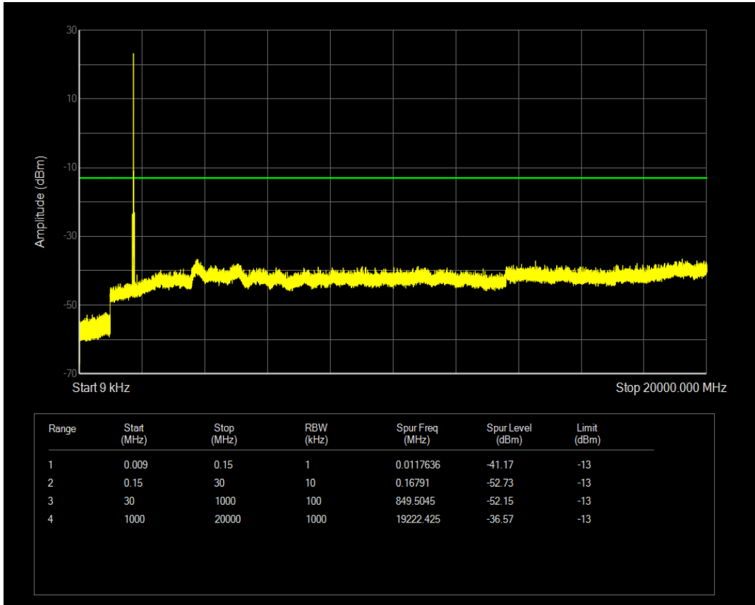
n66 SCS=15kHz DFT_QPSK BW=5MHz Channel=349000 RB=1@24
