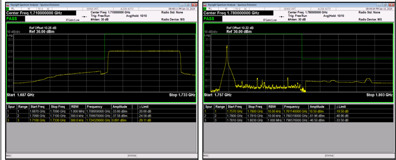
Band66-20MHz-64QAM-132572-1RB#99
