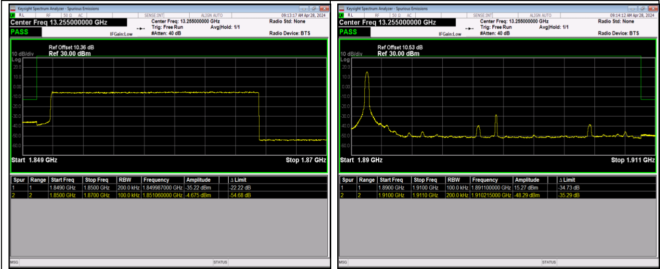
Band2_20MHz_64QAM_18700_100RB#0
