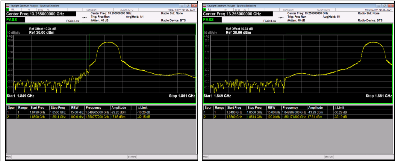
Band2_1.4MHz_64QAM_18607_1RB#0
