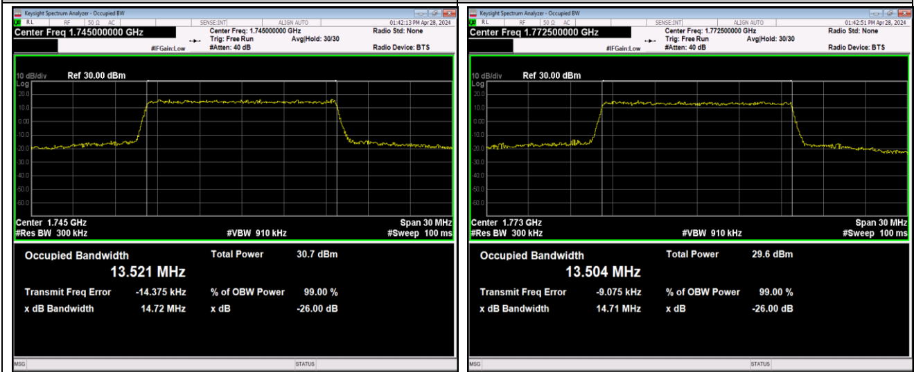
Band66-15MHz-16QAM-132322-75RB#0-PASS
