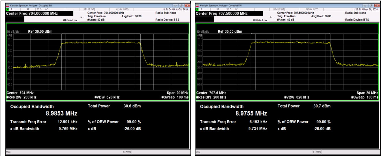
Band12-10MHz-16QAM-23060-50RB#0-PASS
