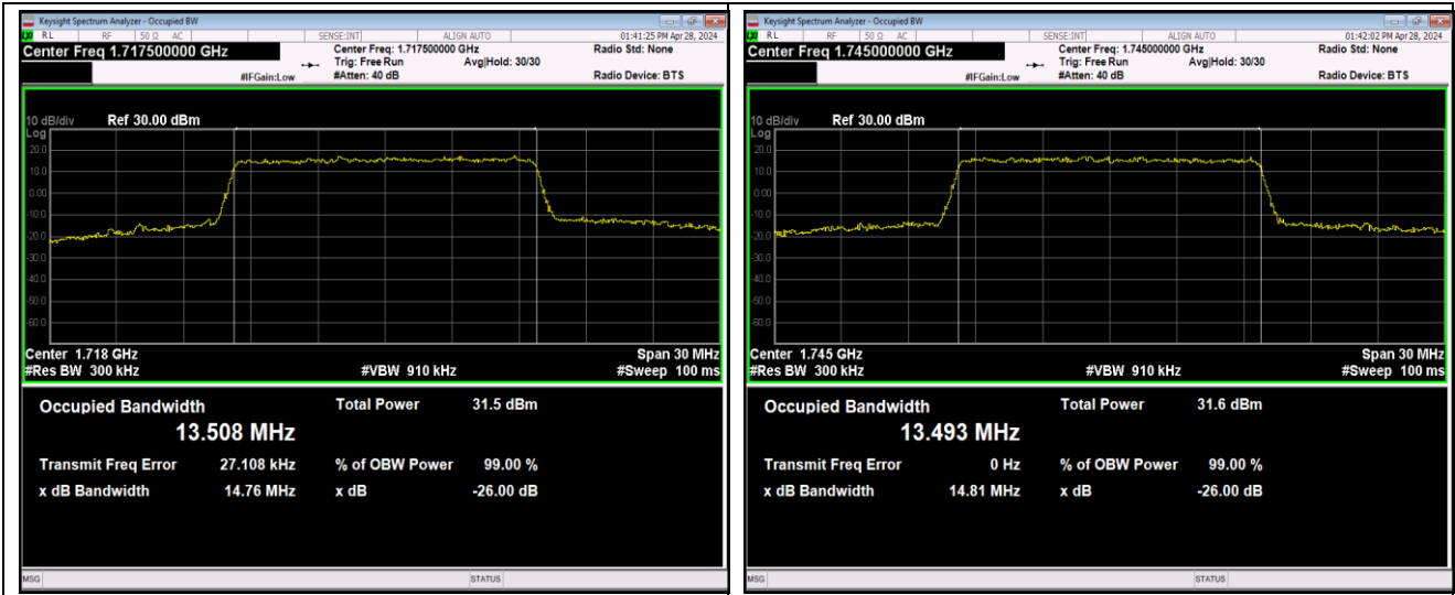
Band66-15MHz-QPSK-132047-75RB#0-PASS
