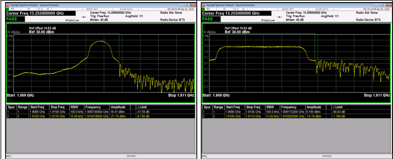
Band2_1.4MHz_QPSK_19193_1RB#5
