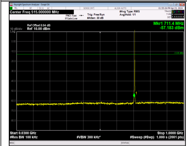
Band12_1.4MHz_16QAM_23173_1RB#0_30~1000_30~1000
