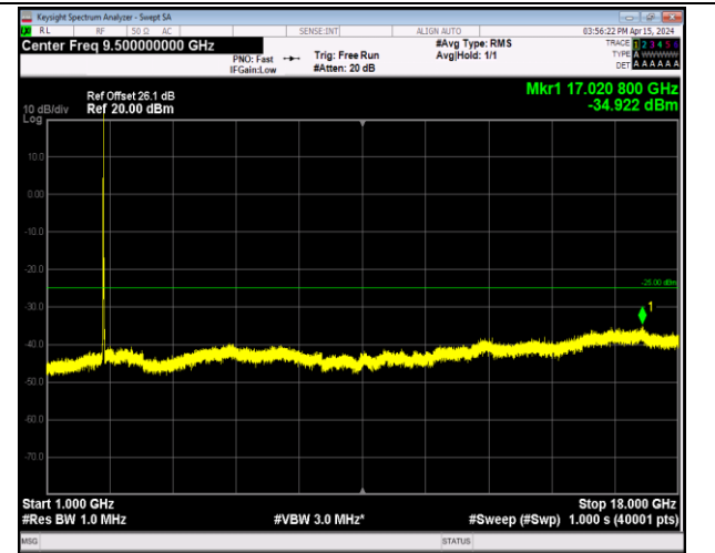
Band7_20MHz_64QAM_21100_1RB#0_1000~18000_100 0~18000
