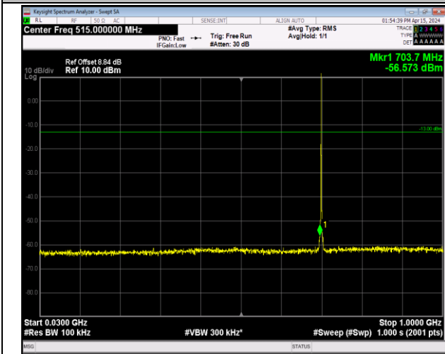
Band12_1.4MHz_64QAM_23095_1RB#0_30~1000_30~1000
