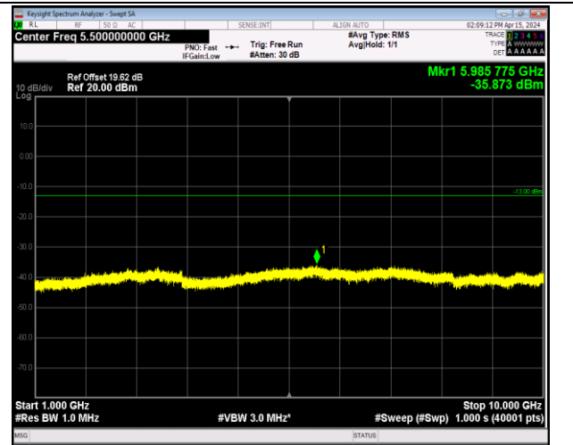
Band12_10MHz_QPSK_23060_1RB#0_1000~10000_100 0~10000
