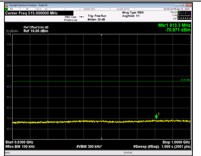
Band7_20MHz_16QAM_21100_1RB#0_30~1000_30~100 0
