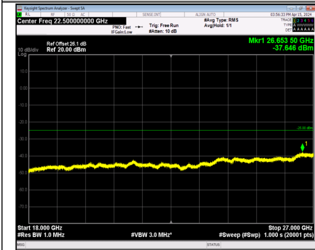
Band7_20MHz_64QAM_21100_1RB#0_18000~27000_18 000~27000
