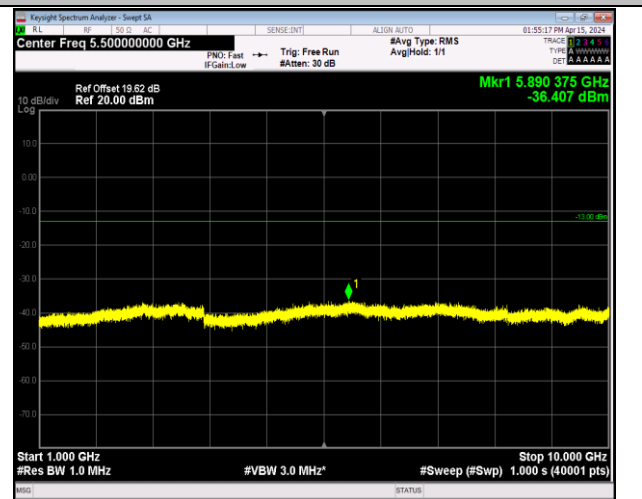
Band12_1.4MHz_QPSK_23173_1RB#0_1000~10000_100 0~10000
