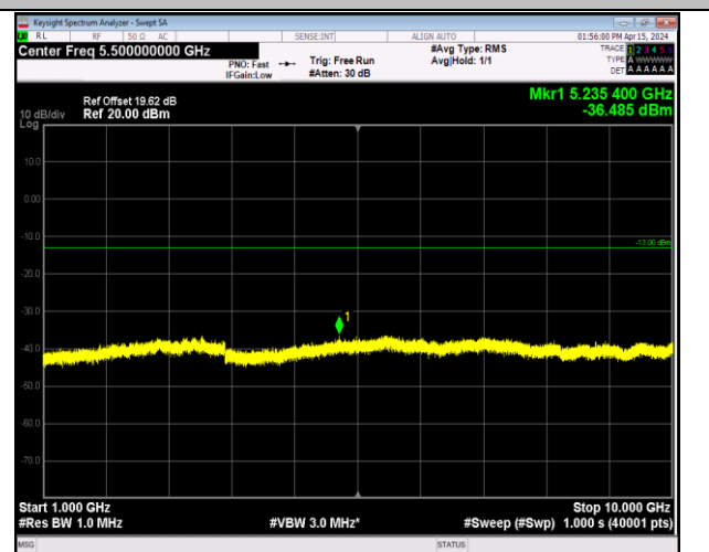
Band12_1.4MHz_64QAM_23173_1RB#0_1000~10000_1000~10000
