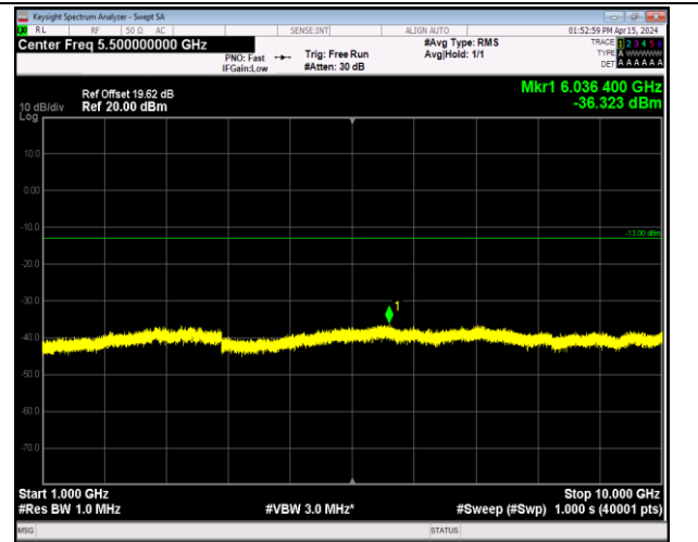
Band12_1.4MHz_QPSK_23017_1RB#0_1000~10000_100 0~10000
