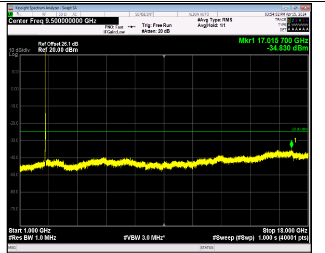
Band7_20MHz_16QAM_20850_1RB#0_1000~18000_100 0~18000
