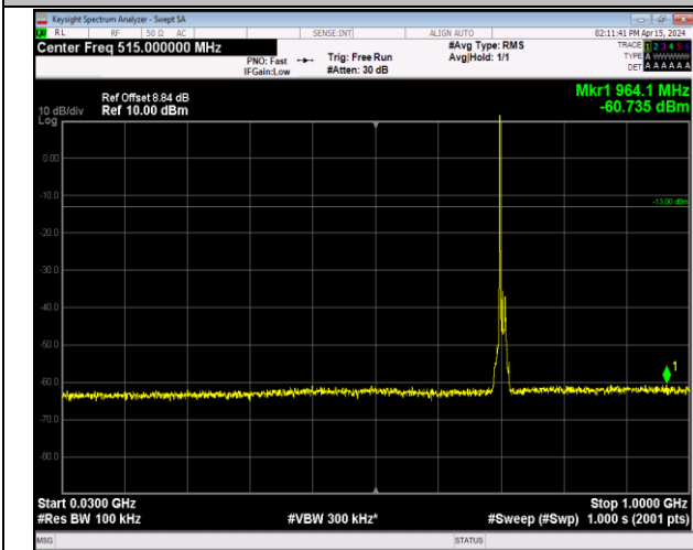
Band12_10MHz_16QAM_23130_1RB#0_30~1000_30~10 00
