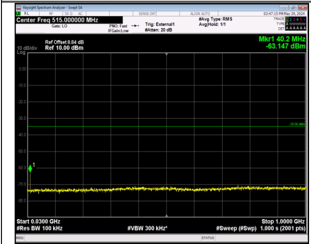
Band38_20MHz_QPSK_38150_1RB#0_30~1000_30~100 0
