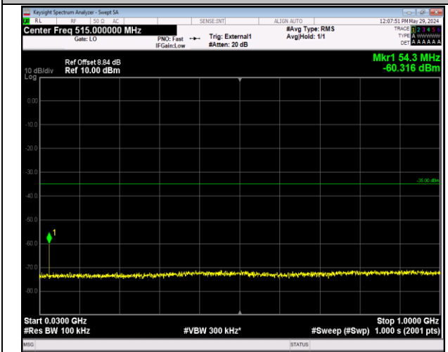
Band38_5MHz_QPSK_38225_1RB#0_30~1000_30~1000
