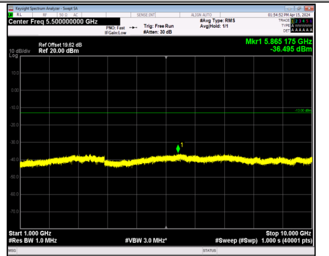
Band12_1.4MHz_64QAM_23095_1RB#0_1000~10000_1000~10000
