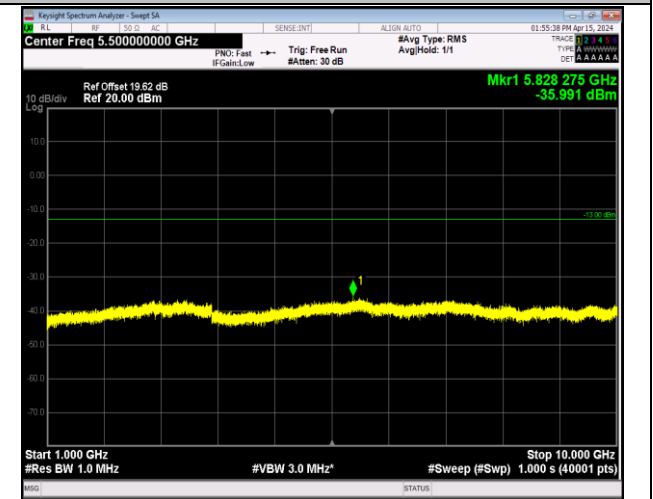
Band12_1.4MHz_16QAM_23173_1RB#0_1000~10000_1000~10000
