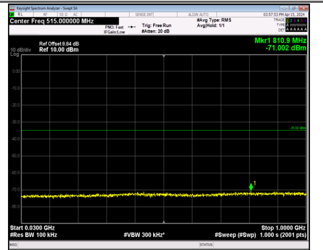
Band7_20MHz_64QAM_21350_1RB#0_30~1000_30~100 0
