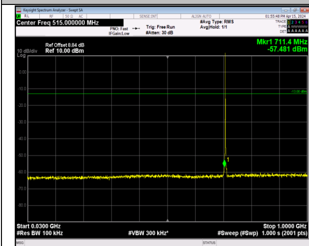
Band12_1.4MHz_64QAM_23173_1RB#0_30~1000_30~1000
