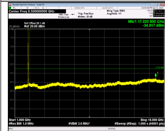
Band7_20MHz_16QAM_21100_1RB#0_1000~18000_100 0~18000
