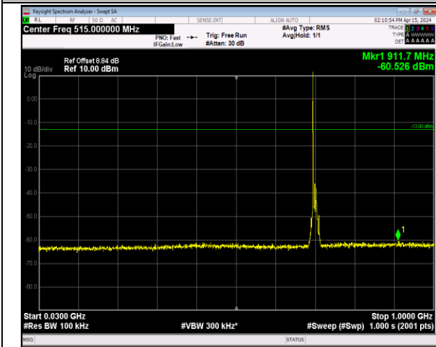
Band12_10MHz_64QAM_23095_1RB#0_30~1000_30~10 00
