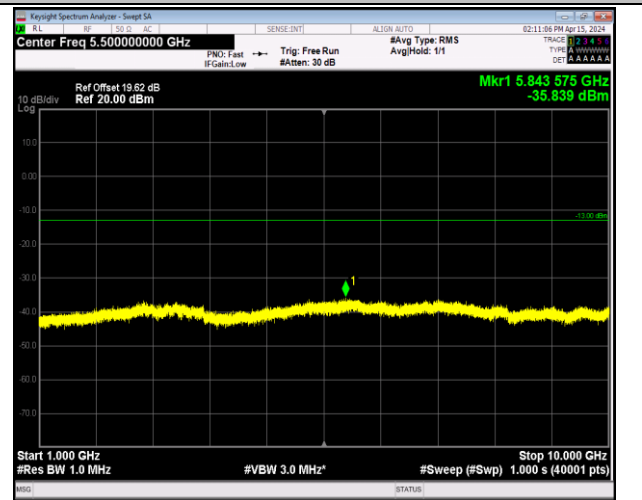
Band12_10MHz_64QAM_23095_1RB#0_1000~10000_10 00~10000
