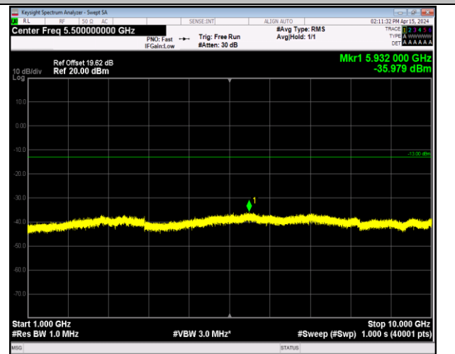
Band12_10MHz_QPSK_23130_1RB#0_1000~10000_100 0~10000
