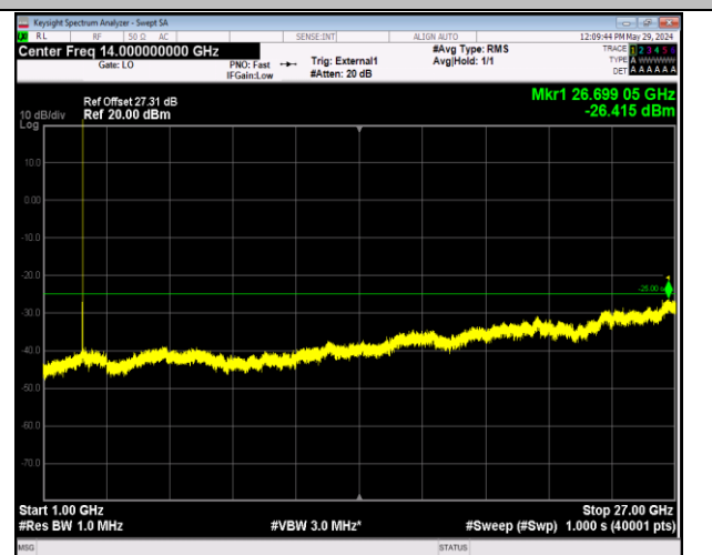
Band38_5MHz_64QAM_38225_1RB#0_1000~27000_100 0~27000
