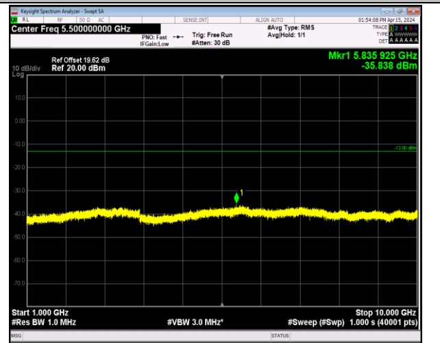
Band12_1.4MHz_QPSK_23095_1RB#0_1000~10000_100 0~10000
