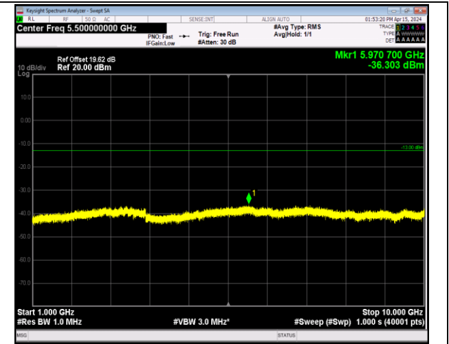
Band12_1.4MHz_16QAM_23017_1RB#0_1000~10000_1000~10000
