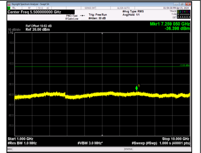
Band12_1.4MHz_16QAM_23095_1RB#0_1000~10000_1000~10000
