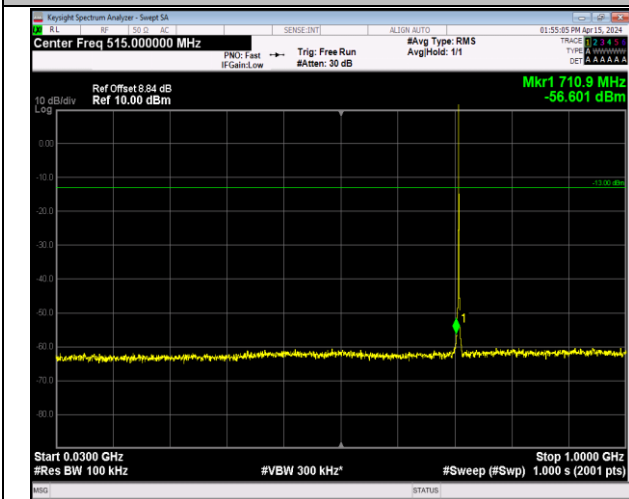
Band12_1.4MHz_QPSK_23173_1RB#0_30~1000_30~100 0
