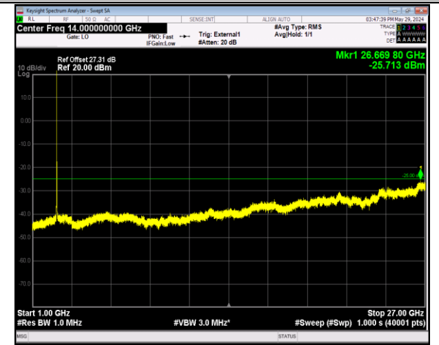
Band38_20MHz_QPSK_38150_1RB#0_1000~27000_100 0~27000
