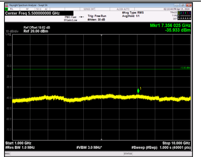
Band12_10MHz_16QAM_23095_1RB#0_1000~10000_10 00~10000
