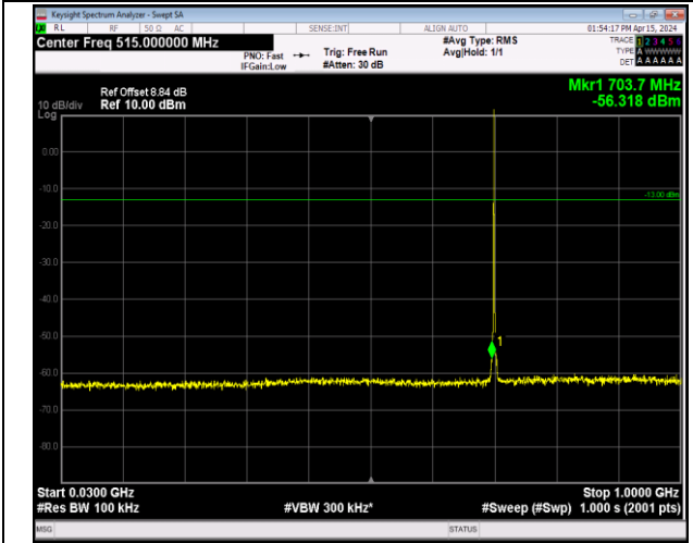
Band12_1.4MHz_16QAM_23095_1RB#0_30~1000_30~1000
