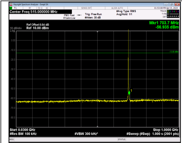
Band12_1.4MHz_16QAM_23017_1RB#0_30~1000_30~1000
