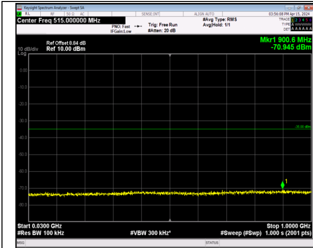
Band7_20MHz_64QAM_21100_1RB#0_30~1000_30~100 0
