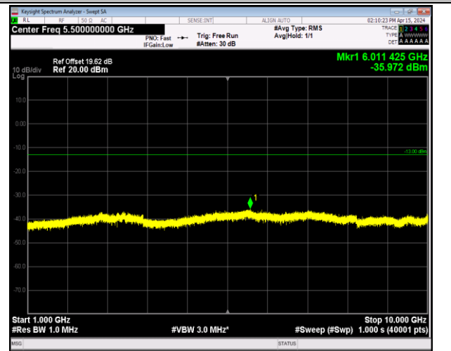
Band12_10MHz_QPSK_23095_1RB#0_1000~10000_100 0~10000
