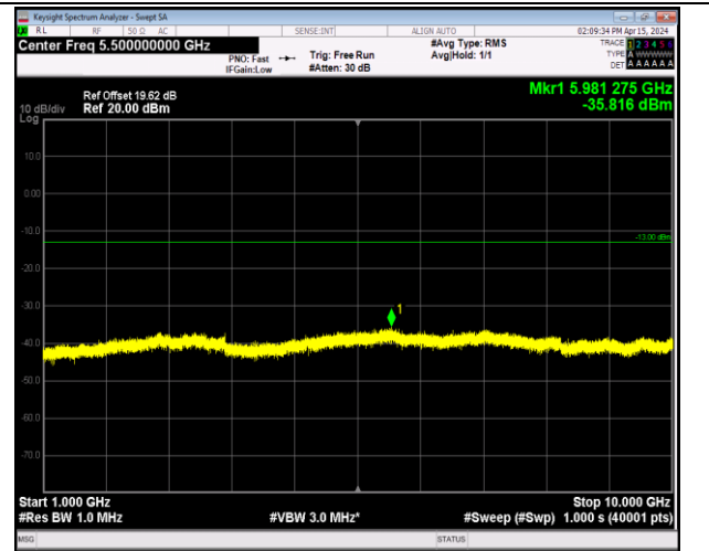
Band12_10MHz_16QAM_23060_1RB#0_1000~10000_10 00~10000
