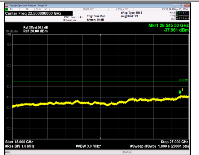
Band7_20MHz_16QAM_21100_1RB#0_18000~27000_18 000~27000
