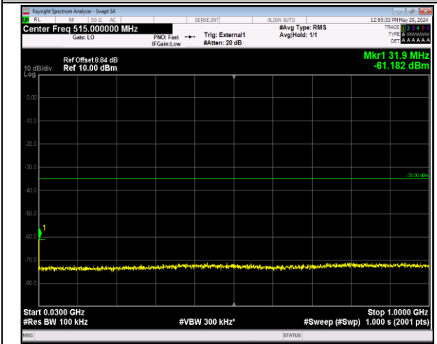
Band38_5MHz_QPSK_38000_1RB#0_30~1000_30~1000
