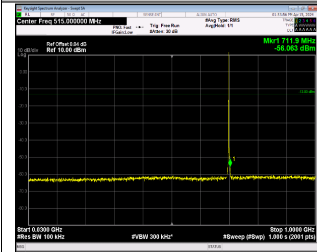
Band12_1.4MHz_QPSK_23095_1RB#0_30~1000_30~100 0
