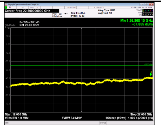
Band7_20MHz_64QAM_21350_1RB#0_18000~27000_18 000~27000
