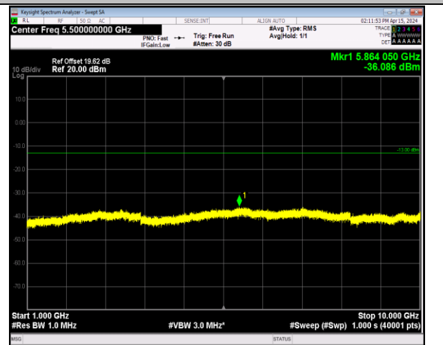
Band12_10MHz_16QAM_23130_1RB#0_1000~10000_10 00~10000
