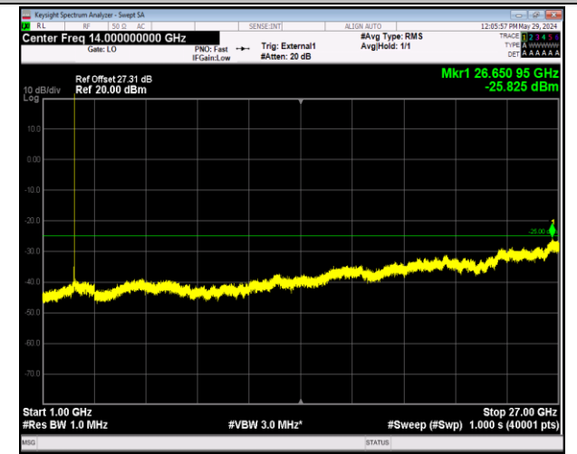
Band38_5MHz_QPSK_38000_1RB#0_1000~27000_1000~27000
