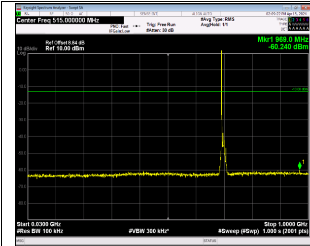
Band12_10MHz_16QAM_23060_1RB#0_30~1000_30~10 00
