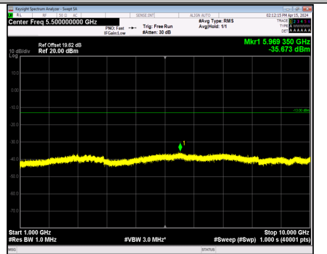
Band12_10MHz_64QAM_23130_1RB#0_1000~10000_10 00~10000
