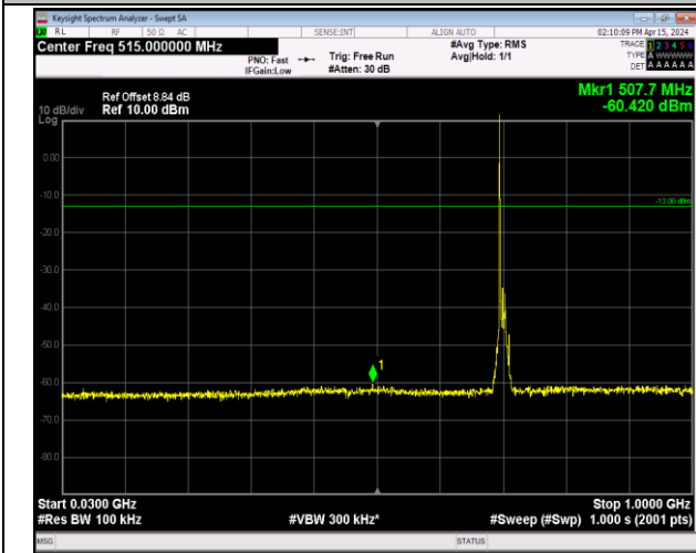
Band12_10MHz_QPSK_23095_1RB#0_30~1000_30~100 0
