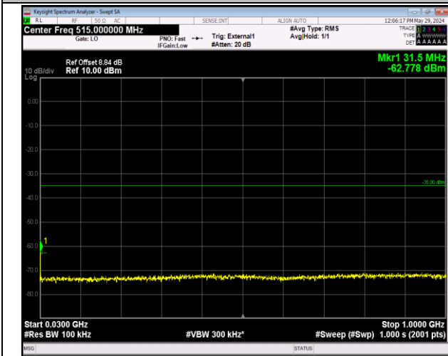
Band38_5MHz_16QAM_38000_1RB#0_30~1000_30~100 0
