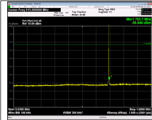
Band12_1.4MHz_QPSK_23017_1RB#0_30~1000_30~100 0
