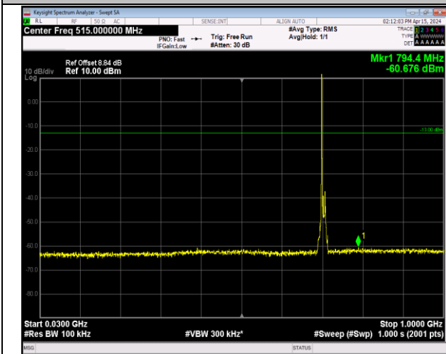
Band12_10MHz_64QAM_23130_1RB#0_30~1000_30~10 00
