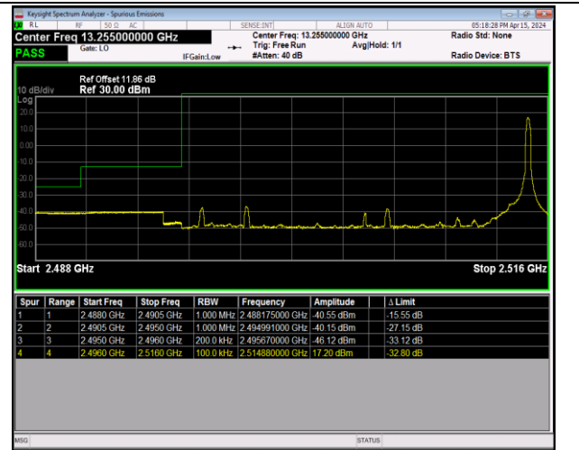
Band41_20MHz_64QAM_39750_1RB#99
