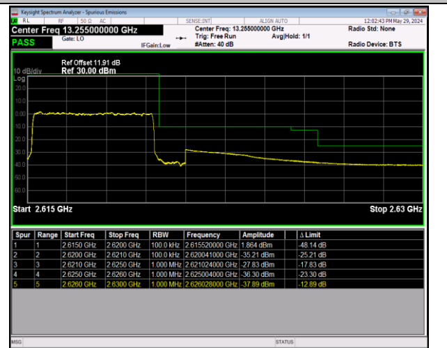
Band38_5MHz_64QAM_38225_25RB#0
