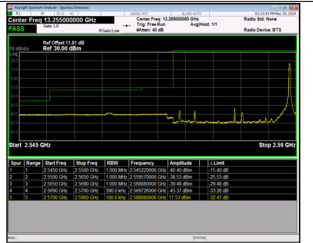
Band38_20MHz_64QAM_37850_1RB#99
