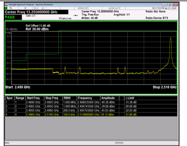
Band41_20MHz_16QAM_39750_1RB#99
