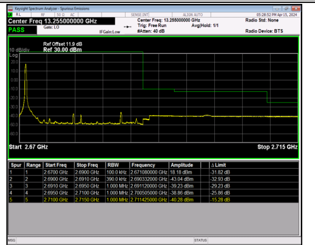
Band41_20MHz_16QAM_41490_1RB#0
