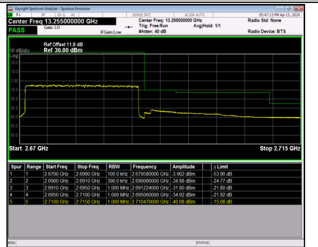
Band41_20MHz_16QAM_41490_100RB#0
