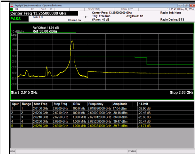
Band38_5MHz_64QAM_38225_1RB#24
