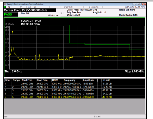
Band38_20MHz_16QAM_38150_1RB#0
