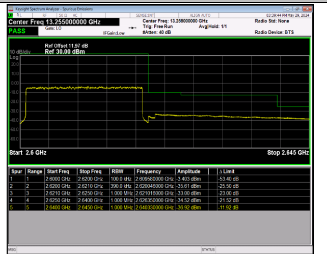
Band38_20MHz_16QAM_38150_100RB#0
