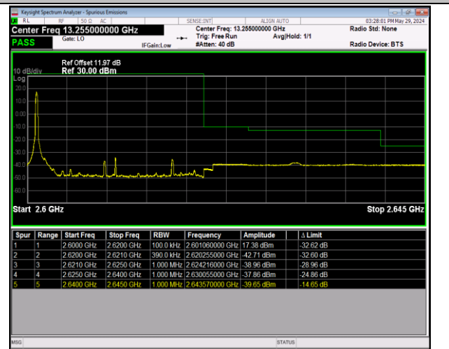
Band38_20MHz_64QAM_38150_1RB#0
