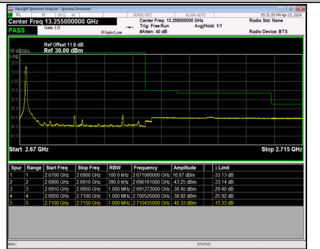
Band41_20MHz_64QAM_41490_1RB#0
