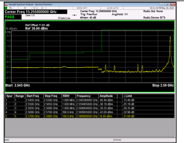
Band38_20MHz_16QAM_37850_1RB#99
