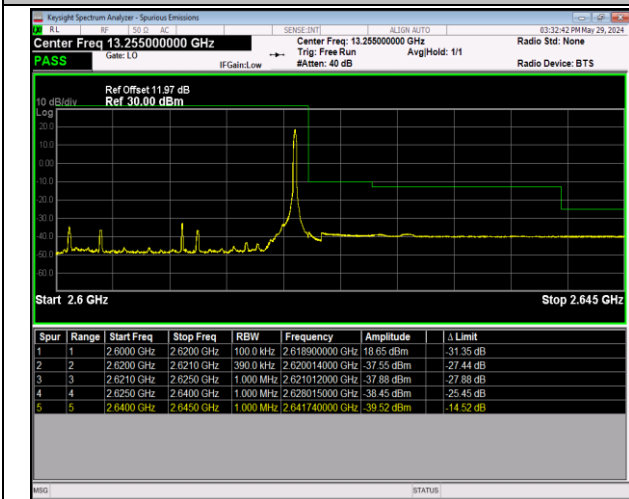
Band38_20MHz_16QAM_38150_1RB#99
