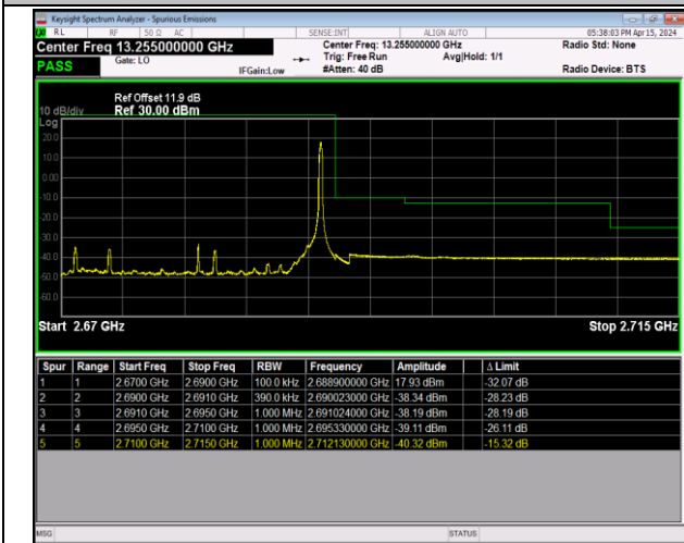
Band41_20MHz_16QAM_41490_1RB#99
