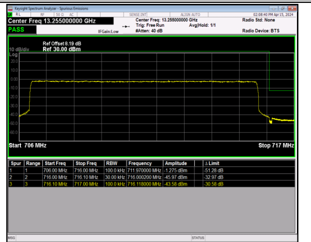
Band12_10MHz_64QAM_23130_50RB#0
