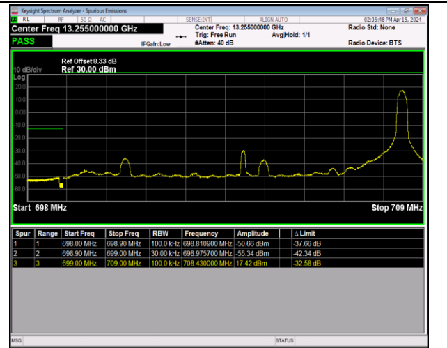
Band12_10MHz_64QAM_23060_1RB#49
