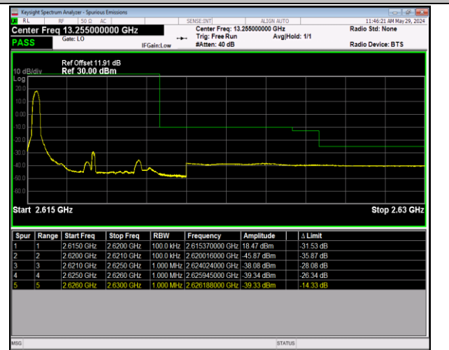
Band38_5MHz_16QAM_38225_1RB#0
