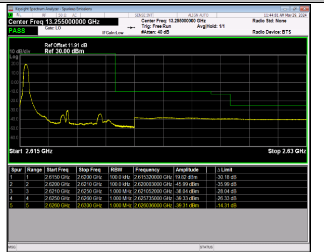
Band38_5MHz_QPSK_38225_1RB#0
