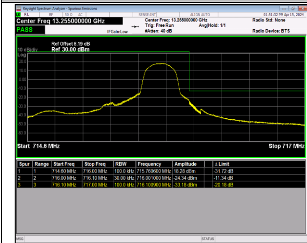
Band12_1.4MHz_16QAM_23173_1RB#0
