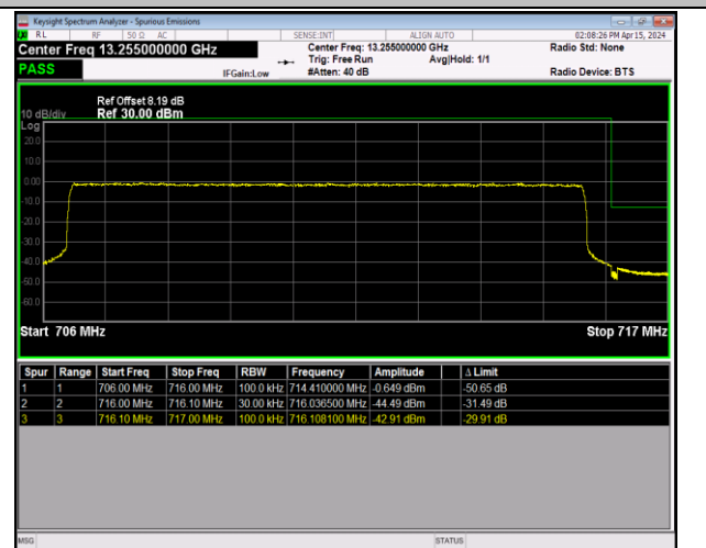
Band12_10MHz_16QAM_23130_50RB#0
