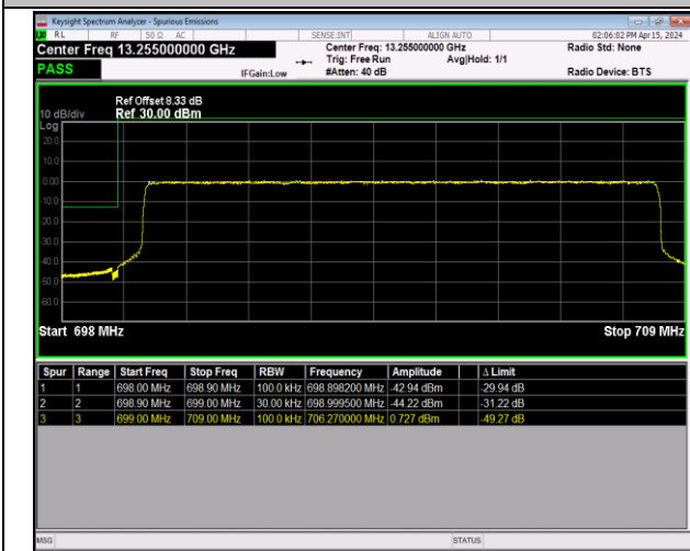
Band12_10MHz_QPSK_23060_50RB#0
