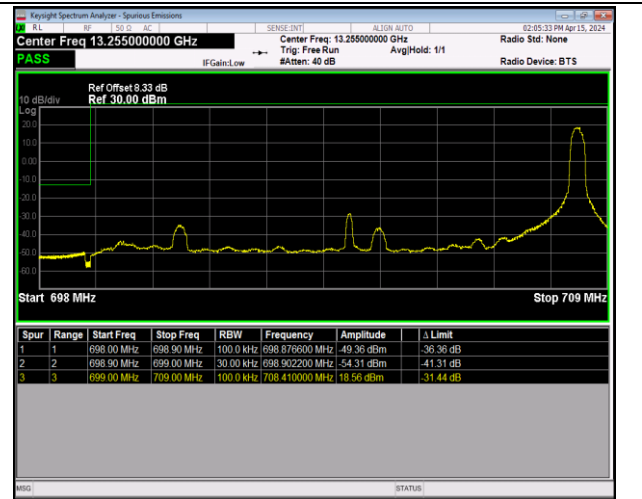
Band12_10MHz_16QAM_23060_1RB#49
