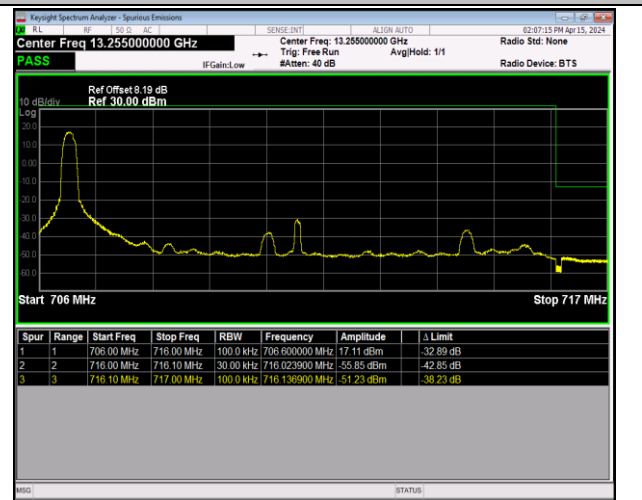
Band12_10MHz_64QAM_23130_1RB#0
