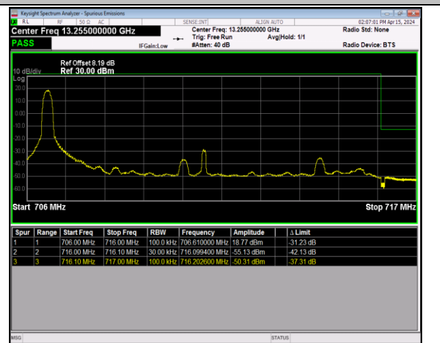
Band12_10MHz_16QAM_23130_1RB#0
