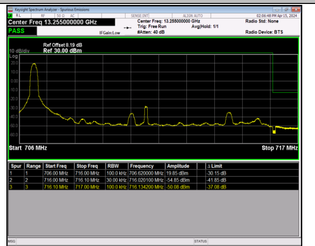
Band12_10MHz_QPSK_23130_1RB#0
