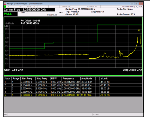
Band38_5MHz_QPSK_37775_1RB#24
