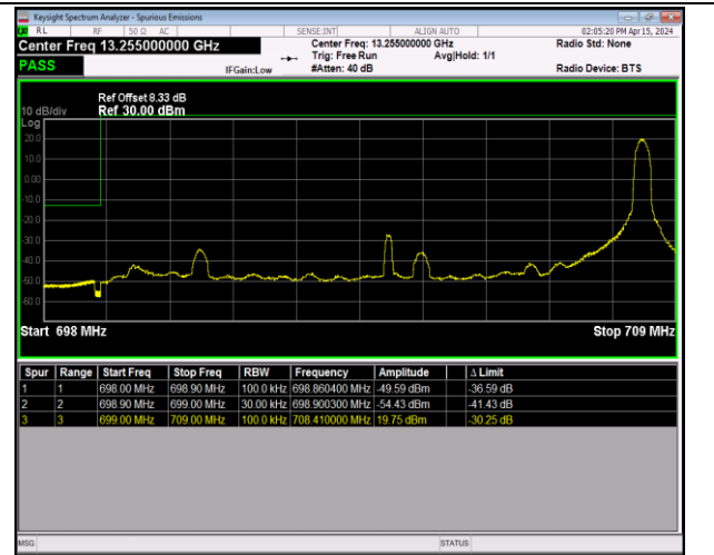
Band12_10MHz_QPSK_23060_1RB#49
