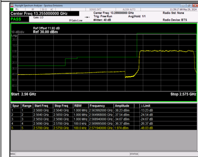
Band38_5MHz_16QAM_3775_25RB#0
