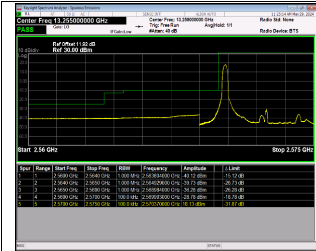
Band38_5MHz_16QAM_3775_1RB#0
