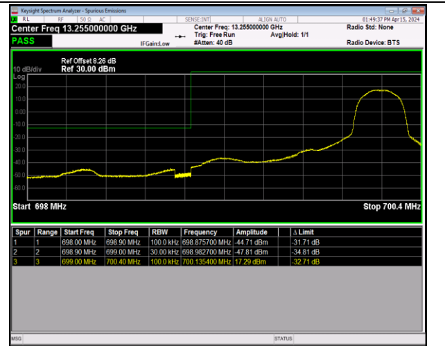
Band12_1.4MHz_64QAM_23017_1RB#5
