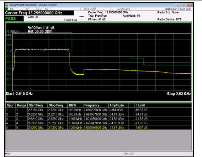
Band38_5MHz_QPSK_38225_25RB#0
