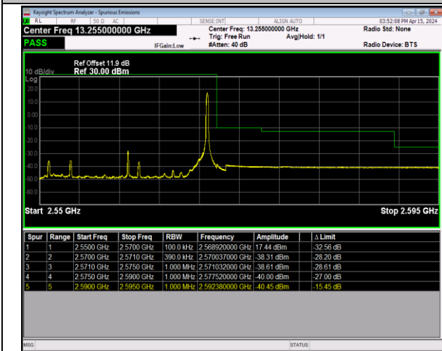
Band7_20MHz_64QAM_21350_1RB#99
