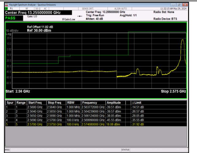
Band38_5MHz_16QAM_3775_1RB#24
