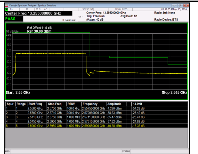
Band7_20MHz_64QAM_21350_100RB#0
