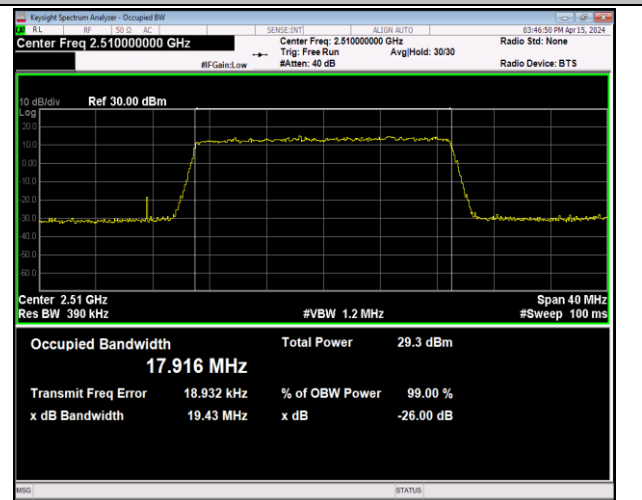
Band7-20MHz-64QAM-20850-100RB#0-PASS
