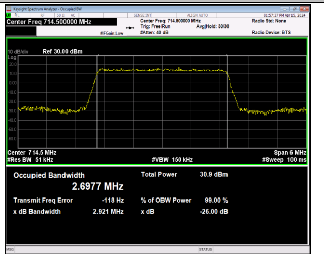
Band12-3MHz-QPSK-23165-15RB#0-PASS
