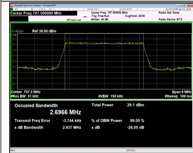
Band12-3MHz-64QAM-23095-15RB#0-PASS
