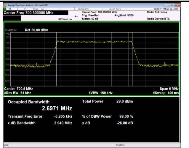
Band12-3MHz-64QAM-23025-15RB#0-PASS
