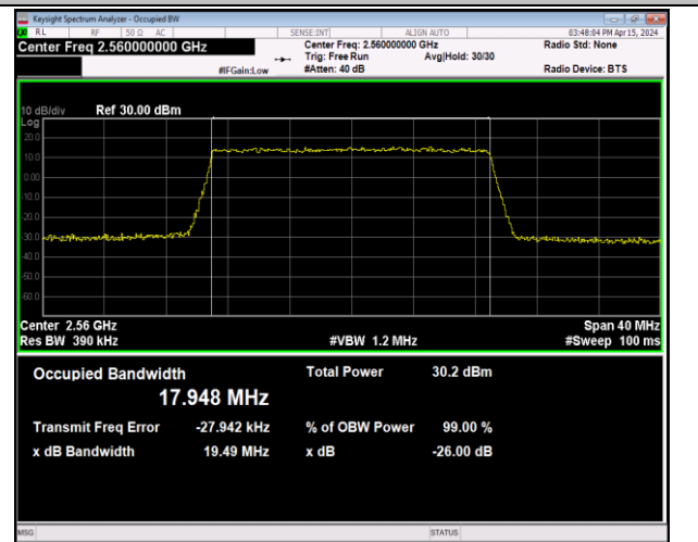
Band7-20MHz-64QAM-21350-100RB#0-PASS
