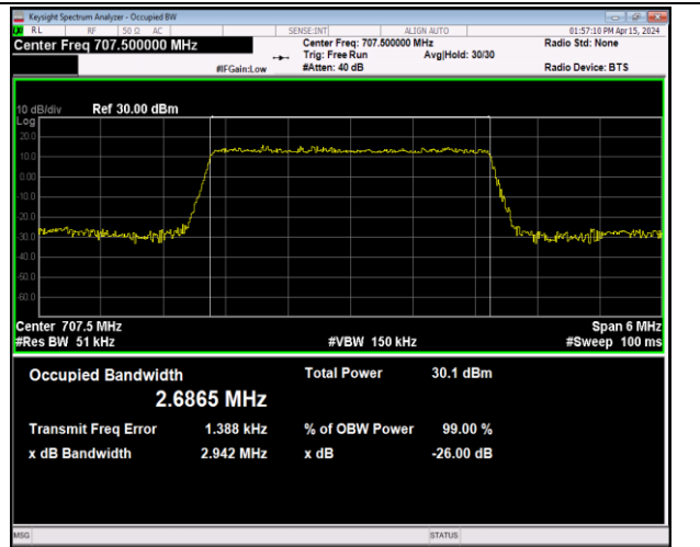
Band12-3MHz-16QAM-23095-15RB#0-PASS
