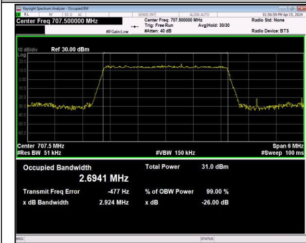
Band12-3MHz-QPSK-23095-15RB#0-PASS
