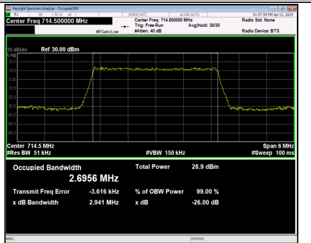
Band12-3MHz-64QAM-23165-15RB#0-PASS
