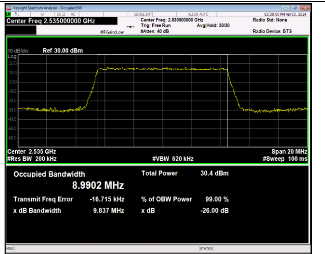
Band7-10MHz-16QAM-21100-50RB#0-PASS
