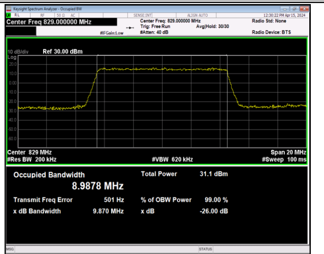
Band5-10MHz-QPSK-20450-50RB#0-PASS
