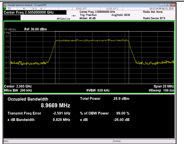
Band7-10MHz-64QAM-20800-50RB#0-PASS
