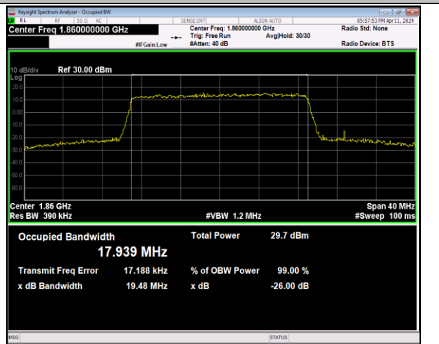
Band2-20MHz-64QAM-18700-100RB#0-PASS
