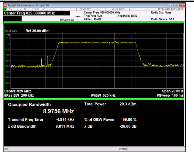
Band5-10MHz-64QAM-20450-50RB#0-PASS
