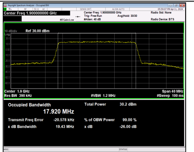
Band2-20MHz-64QAM-19100-100RB#0-PASS
