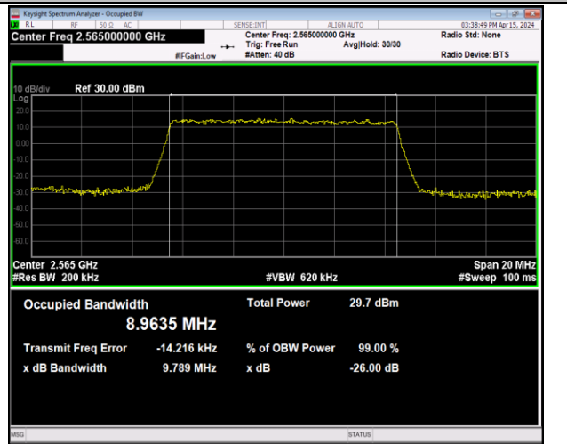
Band7-10MHz-64QAM-21400-50RB#0-PASS
