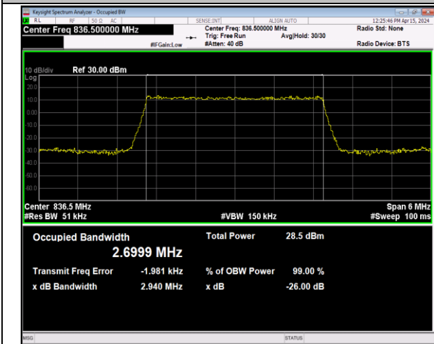
Band5-3MHz-64QAM-20525-15RB#0-PASS
