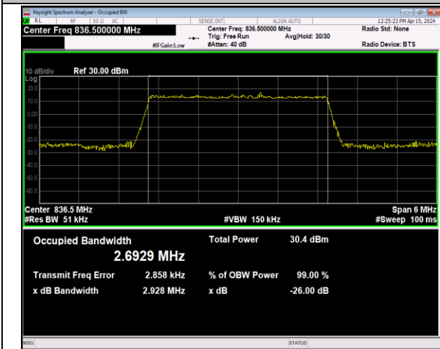
Band5-3MHz-QPSK-20525-15RB#0-PASS
