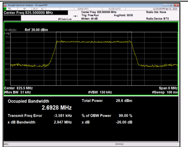
Band5-3MHz-64QAM-20415-15RB#0-PASS
