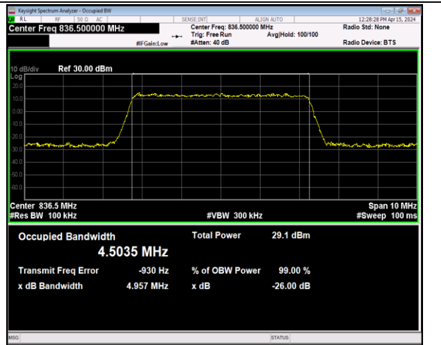
Band5-5MHz-64QAM-20525-25RB#0-PASS
