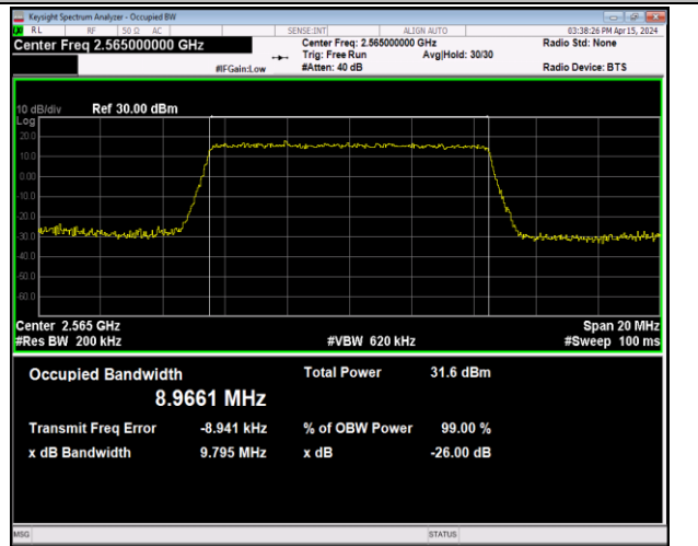
Band7-10MHz-QPSK-21400-50RB#0-PASS
