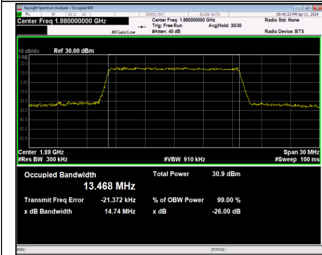
Band2-15MHz-16QAM-18900-75RB#0-PASS
