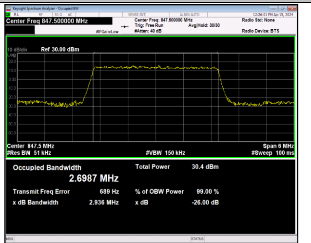
Band5-3MHz-QPSK-20635-15RB#0-PASS
