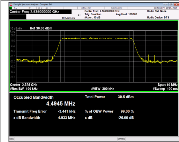
Band7-5MHz-16QAM-21100-25RB#0-PASS
