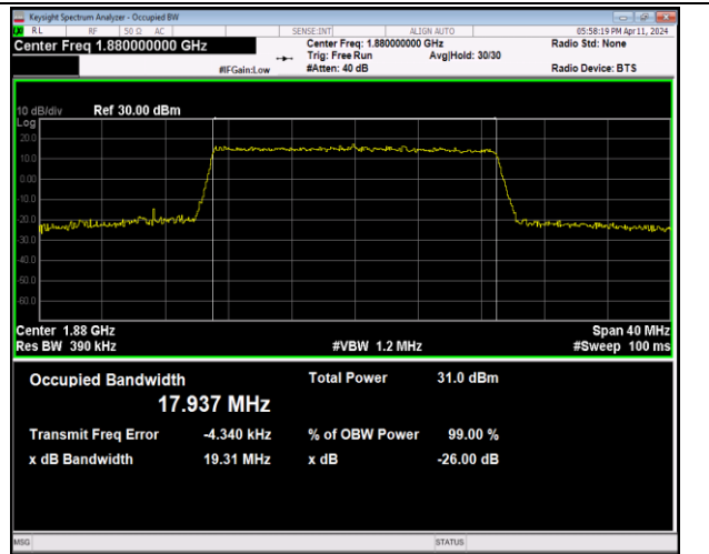
Band2-20MHz-16QAM-18900-100RB#0-PASS
