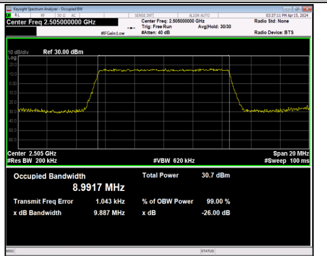
Band7-10MHz-QPSK-20800-50RB#0-PASS
