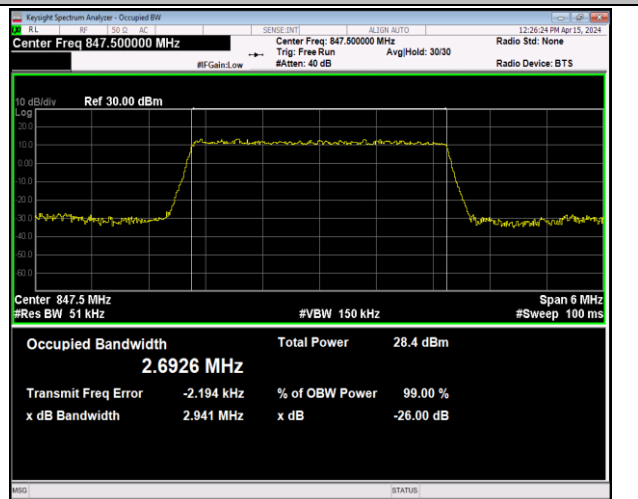
Band5-3MHz-64QAM-20635-15RB#0-PASS
