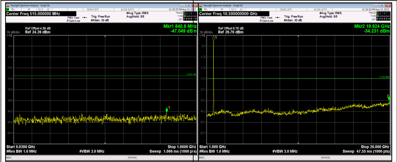
Band4-20MHz-QPSK-20300-1RB#0-Range1:30~1000MHz
