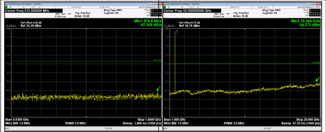
Band4-1.4MHz-64QAM-19957-1RB#0-Range1:30~1000MHz
