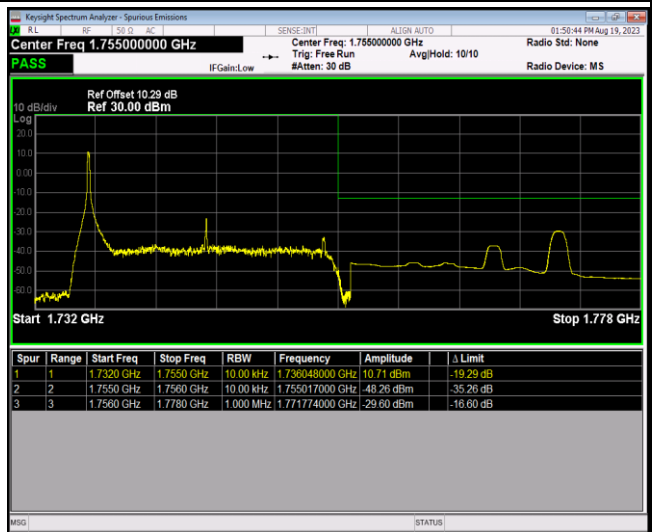
Band4-20MHz-QPSK-20300-100RB#0
