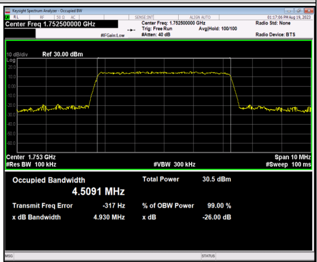
Band4-5MHz-64QAM-20175-25RB#0
