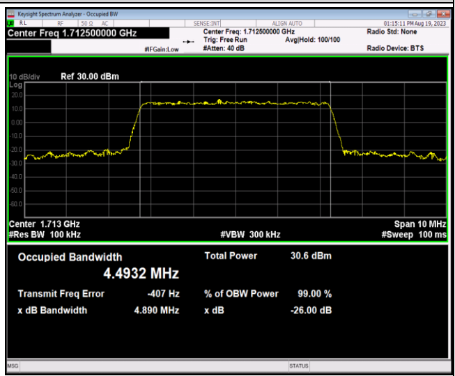
Band4-5MHz-16QAM-20375-25RB#0
