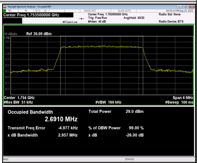
Band4-5MHz-QPSK-20175-25RB#0
