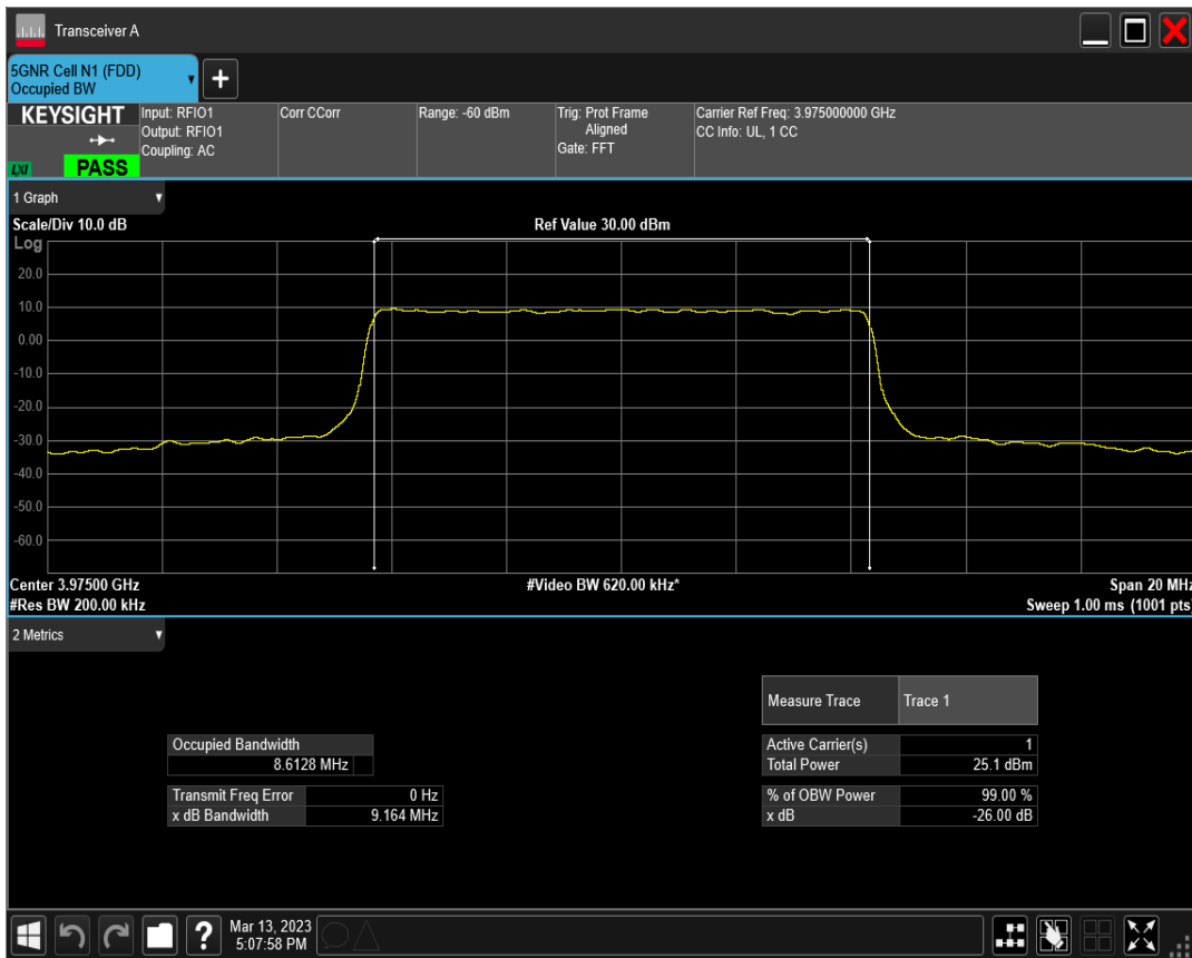
n77(3700-3980) SCS=30kHz DFT_QAM64 BW=10MHz Channel=665000 RB=24@0
