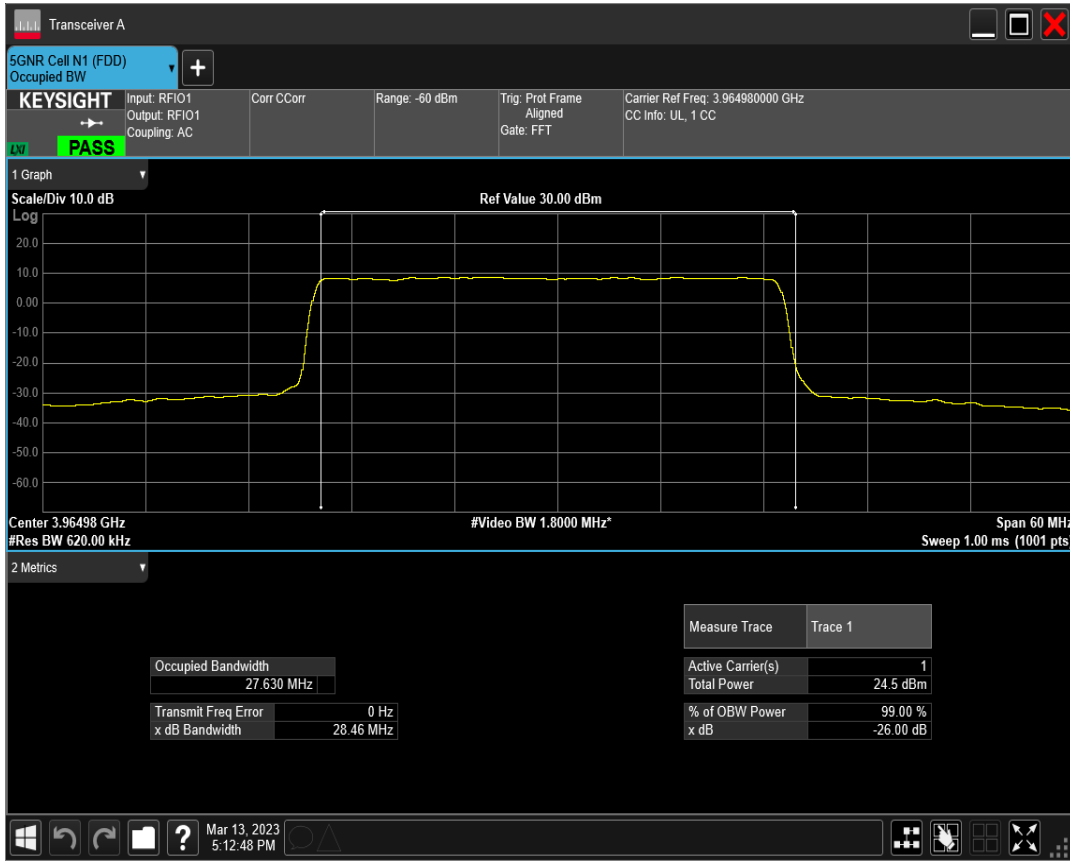
n77(3700-3980) SCS=30kHz DFT_QAM256 BW=30MHz Channel=664332 RB=75@0
