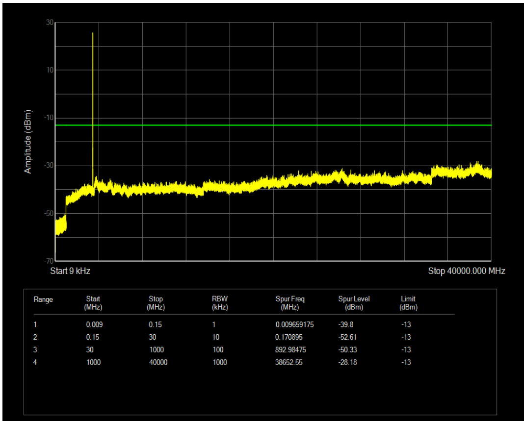
n77(3450-3550) SCS=30kHz DFT_QPSK BW=10MHz Channel=630334 RB=1@0
