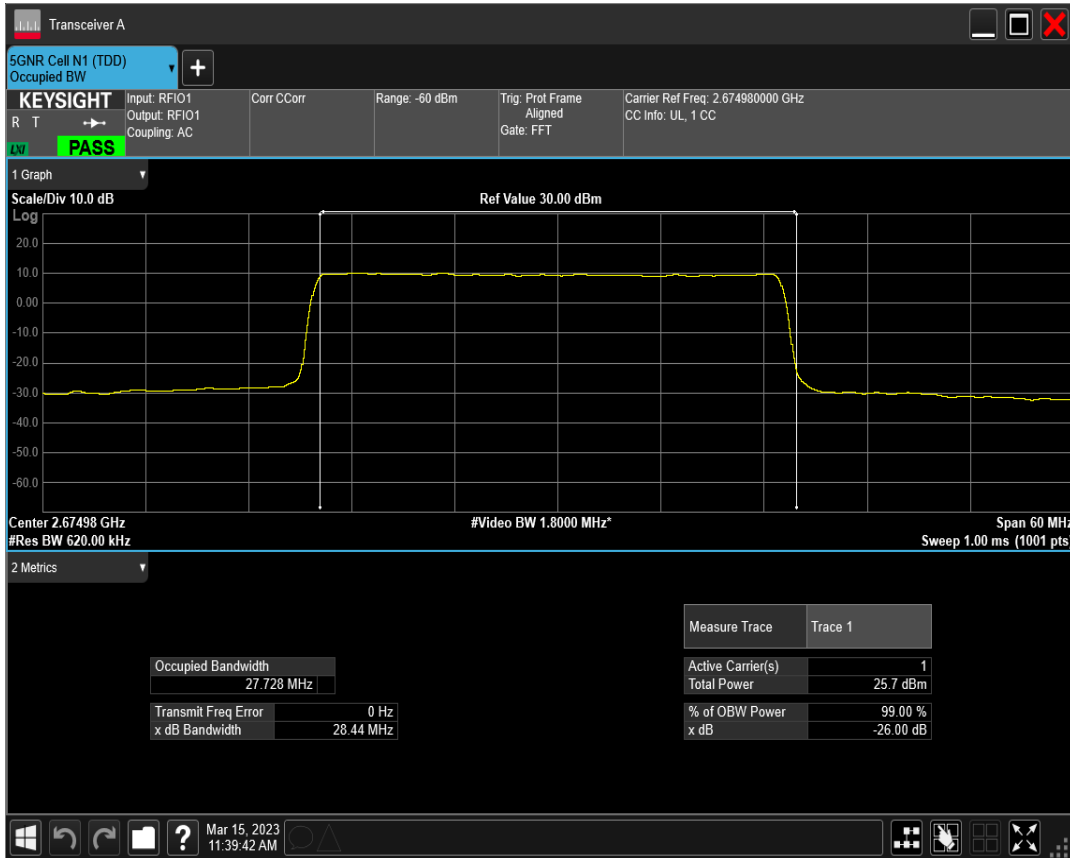
n41 SCS=30kHz DFT_QAM16 BW=30MHz Channel=534996 RB=75@0
