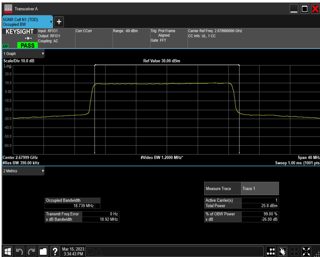
n41 SCS=15kHz DFT_QAM16 BW=20MHz Channel=535998 RB=100@0
