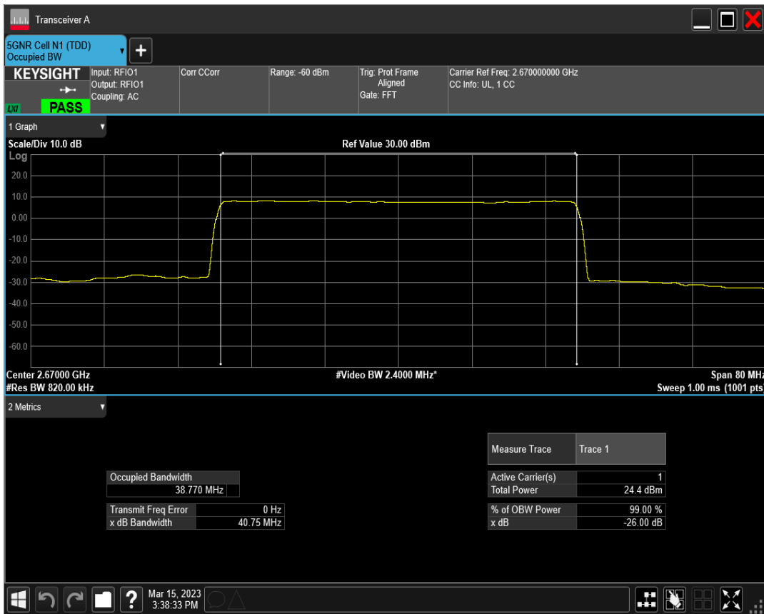
n41 SCS=15kHz DFT_QAM256 BW=40MHz Channel=534000 RB=216@0
