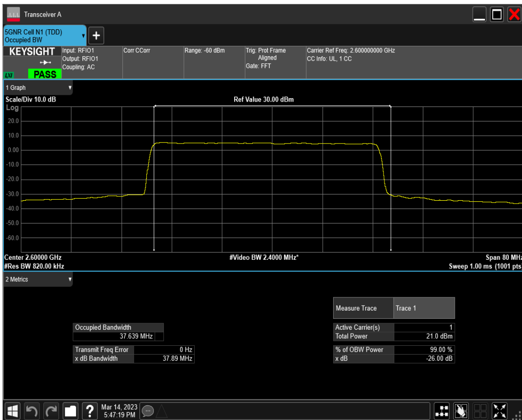
n38 SCS=30kHz DFT_QAM256 BW=40MHz Channel=520000 RB=100@0
