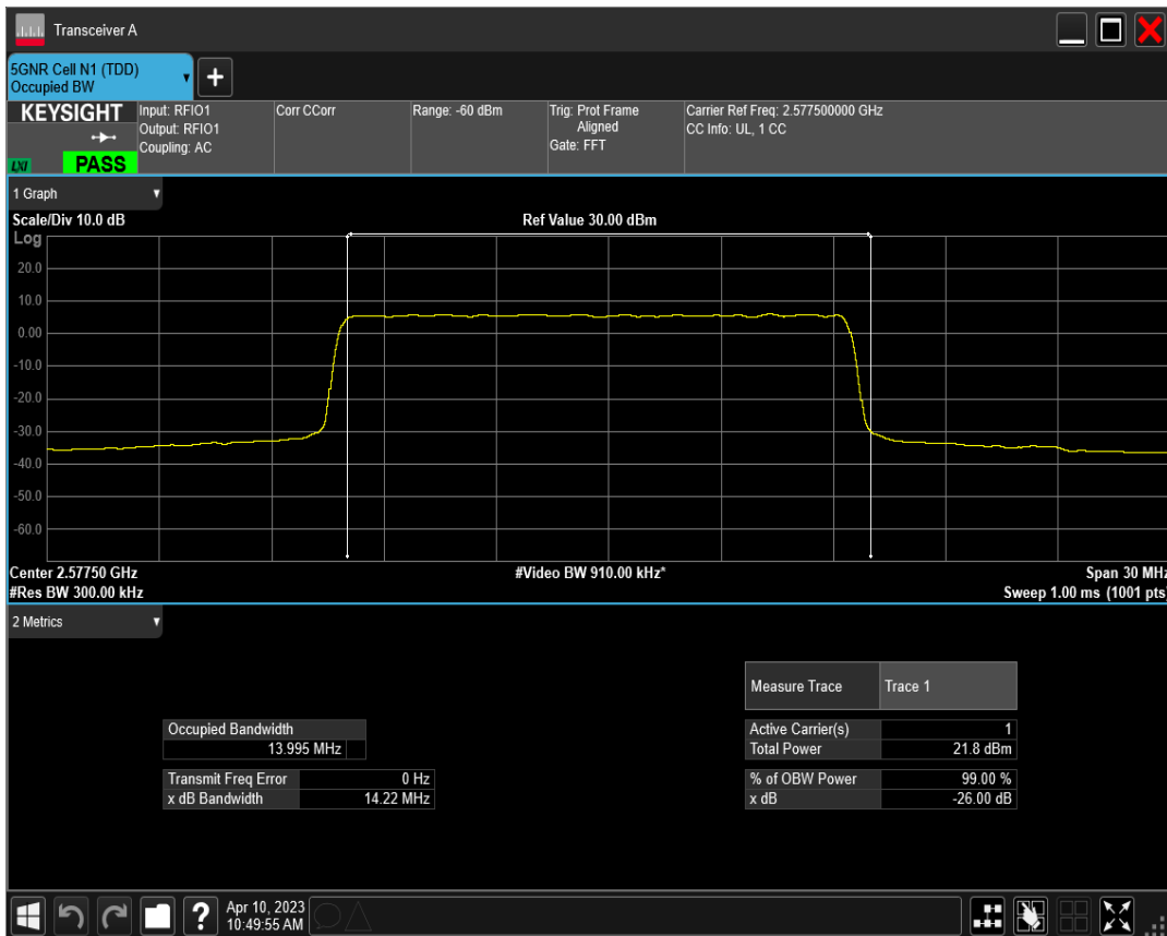
n38 SCS=15kHz DFT_QAM64 BW=15MHz Channel=515500 RB=75@0
