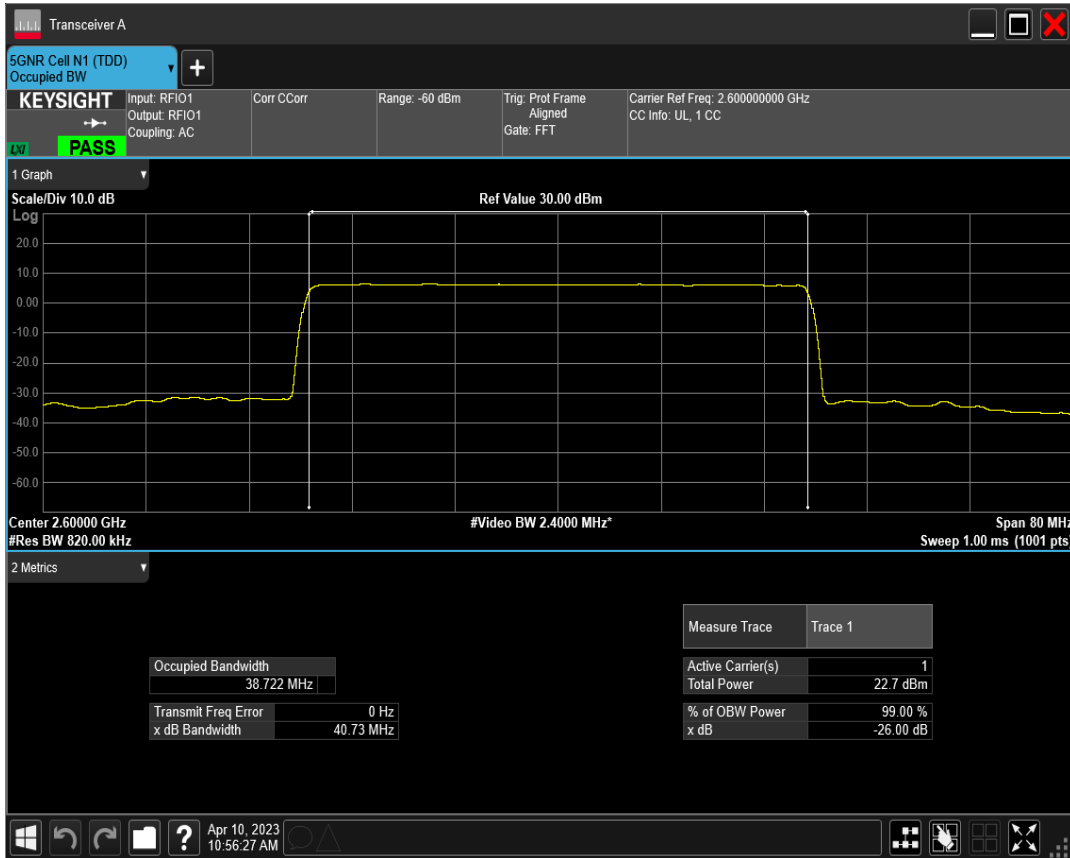
n38 SCS=15kHz DFT_QAM16 BW=40MHz Channel=520000 RB=216@0
