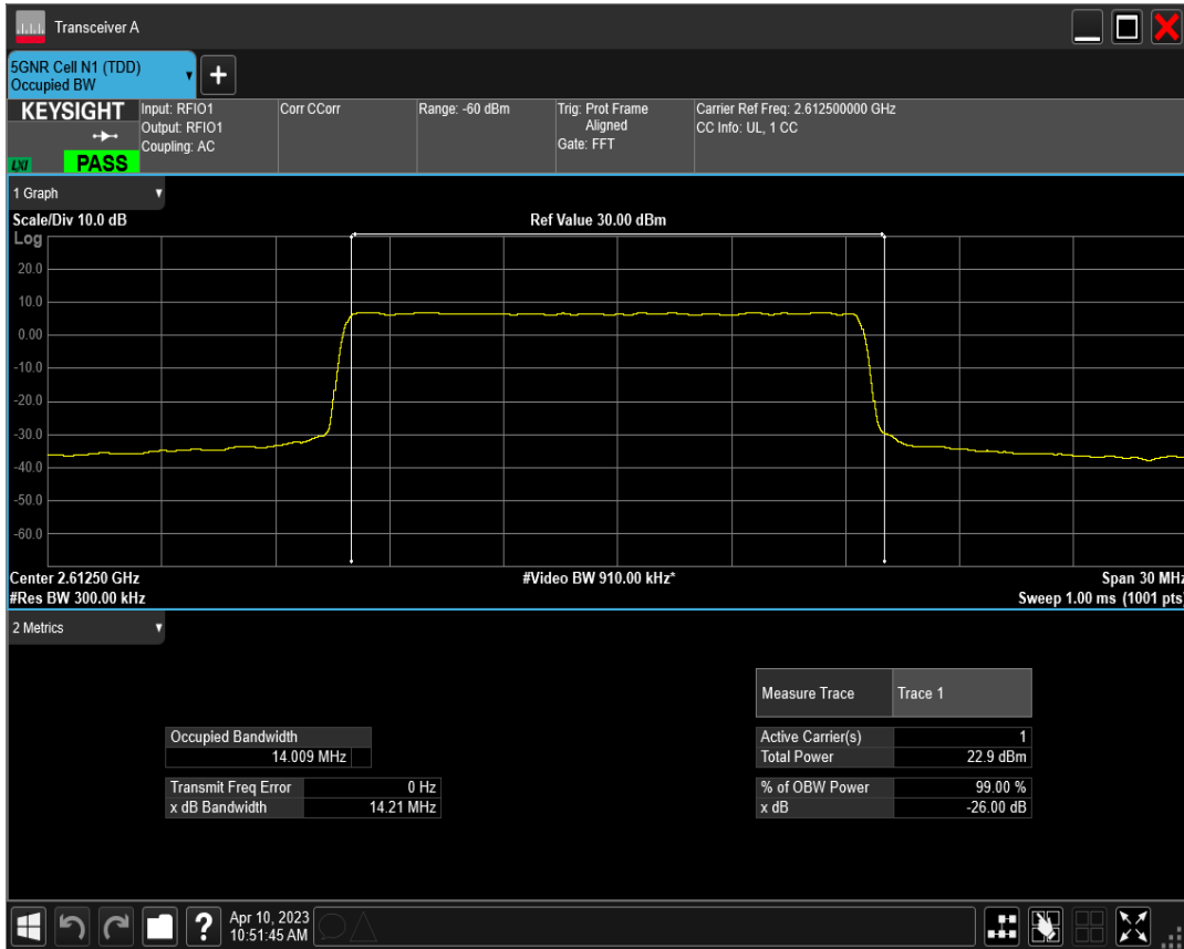
n38 SCS=15kHz DFT_QAM16 BW=15MHz Channel=522500 RB=75@0
