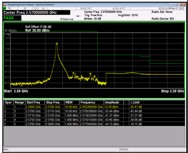
Band7-5MHz-16QAM-21425-25RB#0
