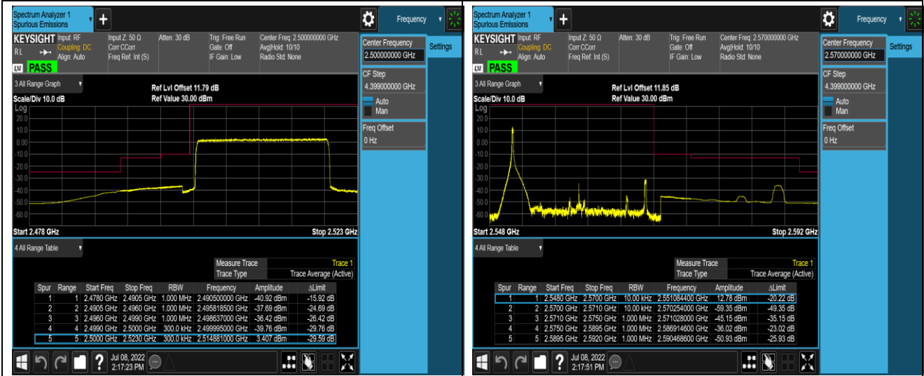
Band7-20MHz-16QAM-21350-1RB#99
