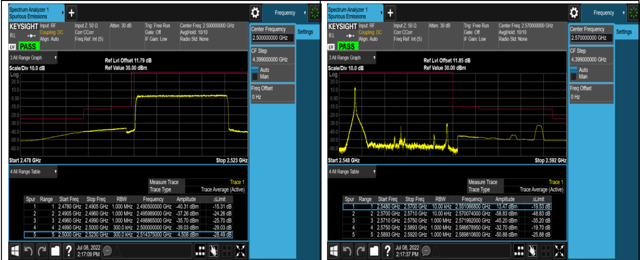
Band7-20MHz-QPSK-21350-1RB#99
