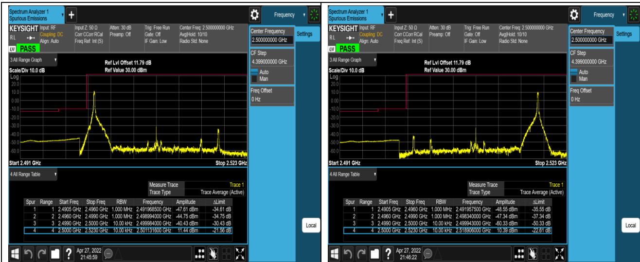
Band7-20MHz-QPSK-2085-100RB#0
