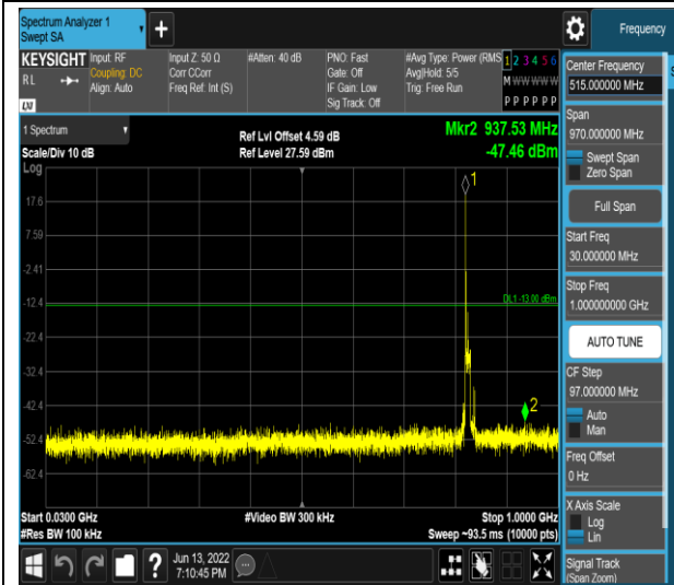
Band5-10MHz-QPSK-20525-1RB#0-Range1:30~1000MHz
