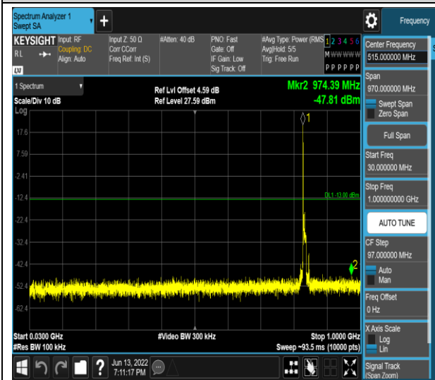
Band5-10MHz-QPSK-20525-1RB#0-Range1:30~1000MHz
