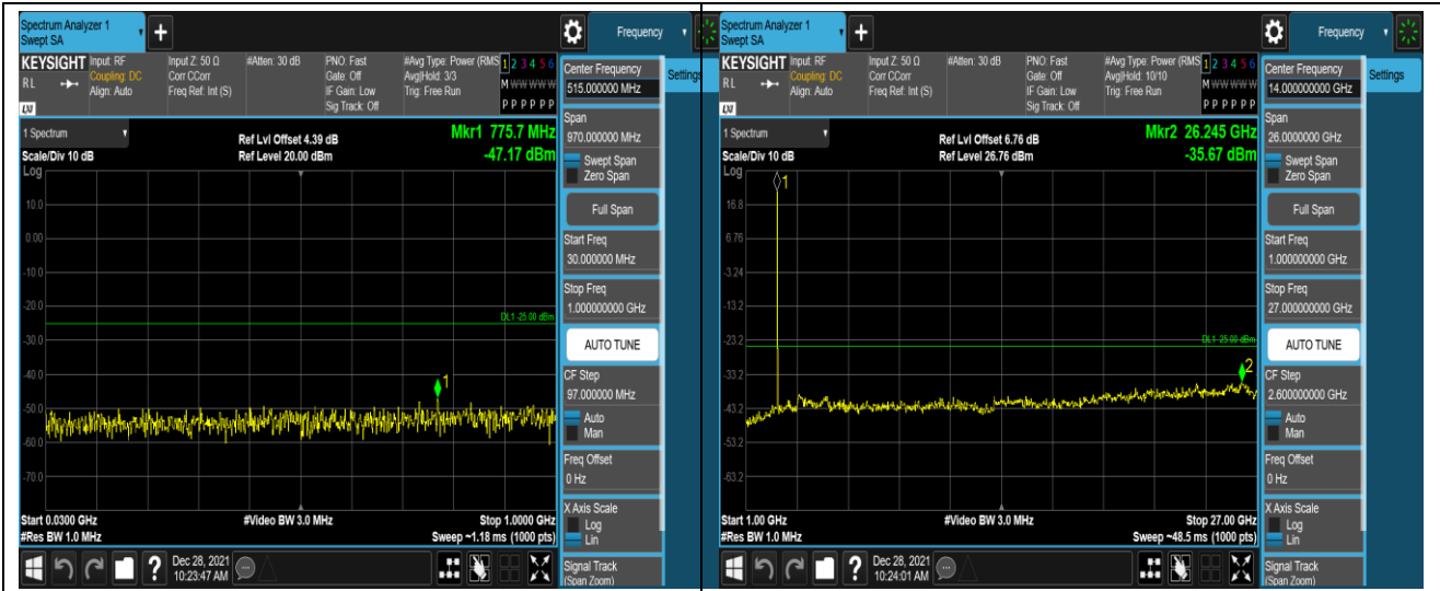
Band38-5MHz-16QAM-38225-1RB#0-Range1:30~1000MHz
