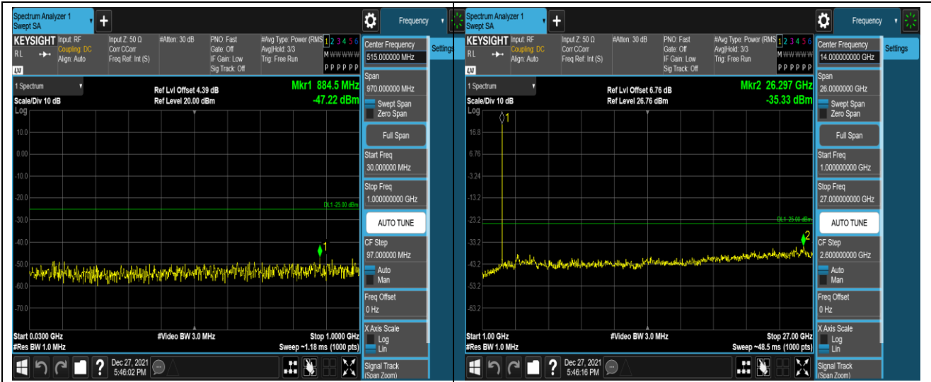
Band38-5MHz-QPSK-37775-1RB#0-Range1:30~1000MHz
