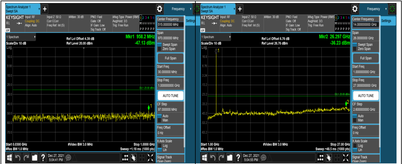
Band7-5MHz-QPSK-21425-1RB#0-Range1:30~1000MHz
