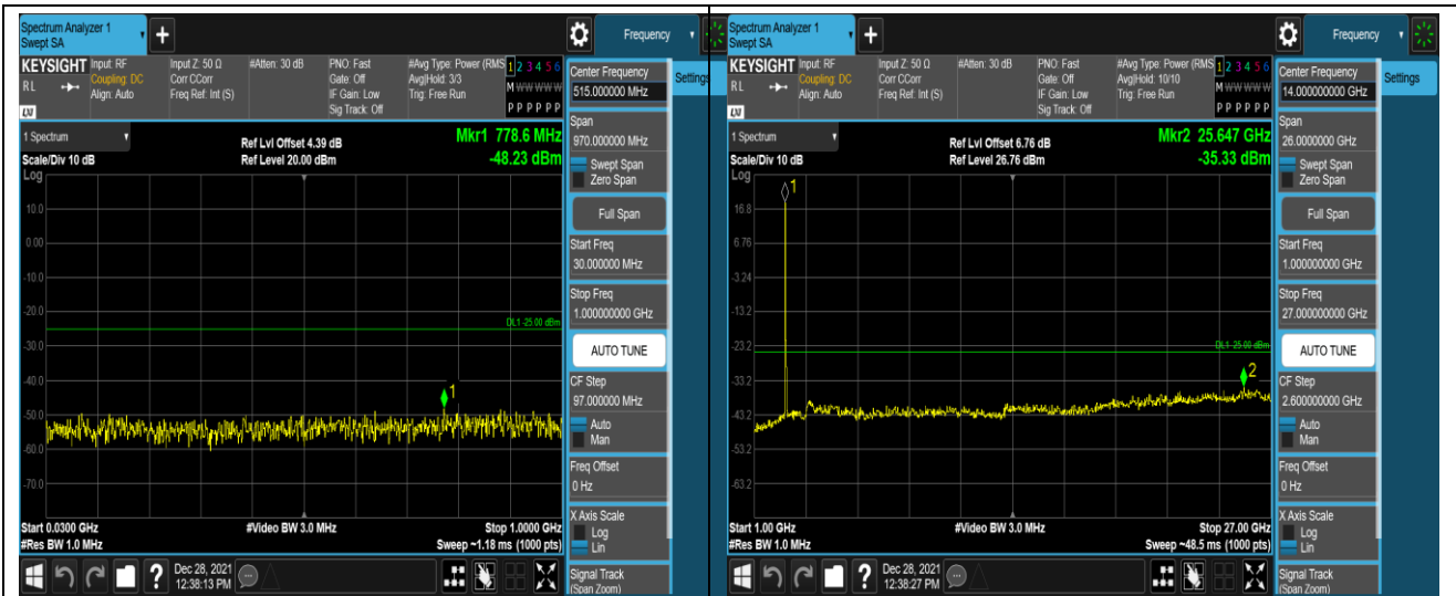
Band38-20MHz-16QAM-38000-1RB#0-Range1:30 ~1000MHz
