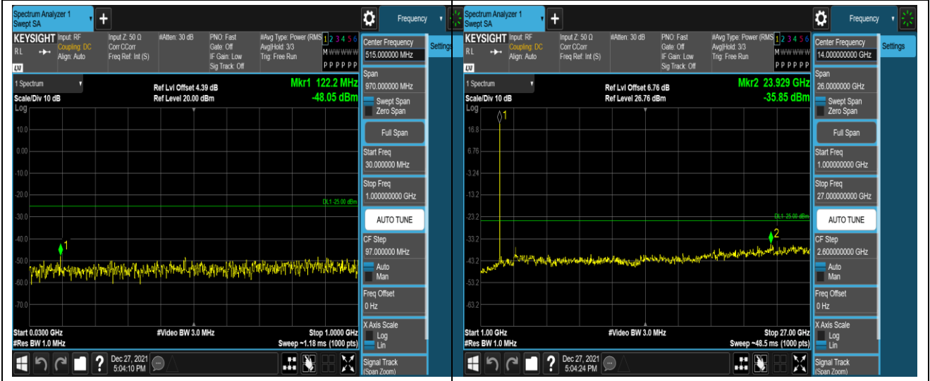
Band7-5MHz-16QAM-20775-1RB#0-Range1:30~1000MHz
