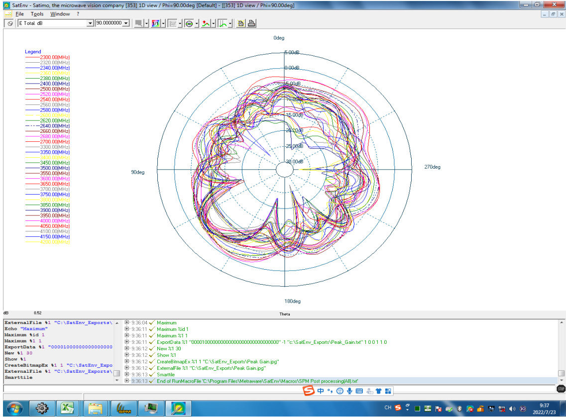
N7/N38/N40/N41/N77/N78 Phi=90deg
