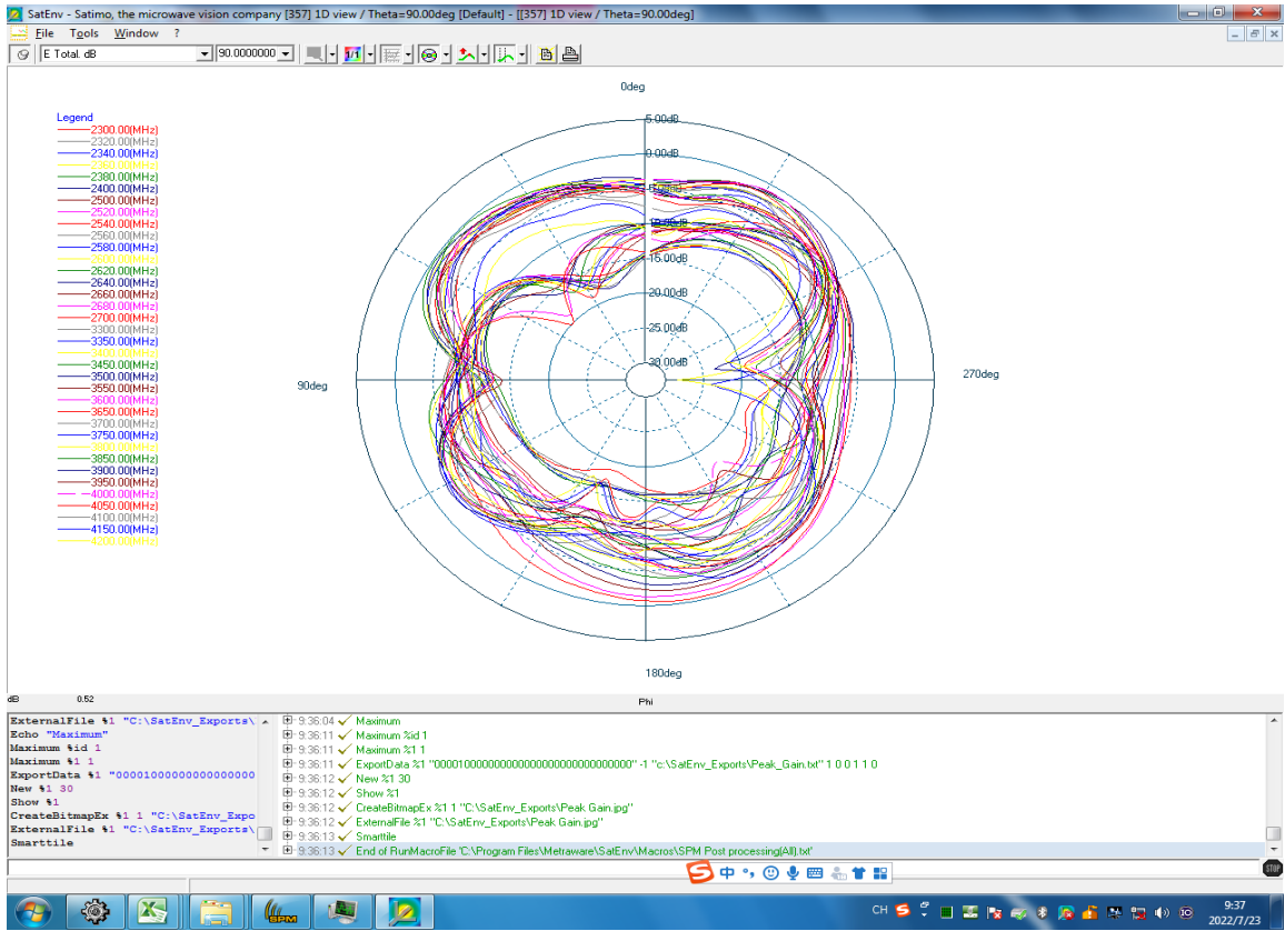
N7/N38/N40/N41/N77/N78 Theta=90deg
