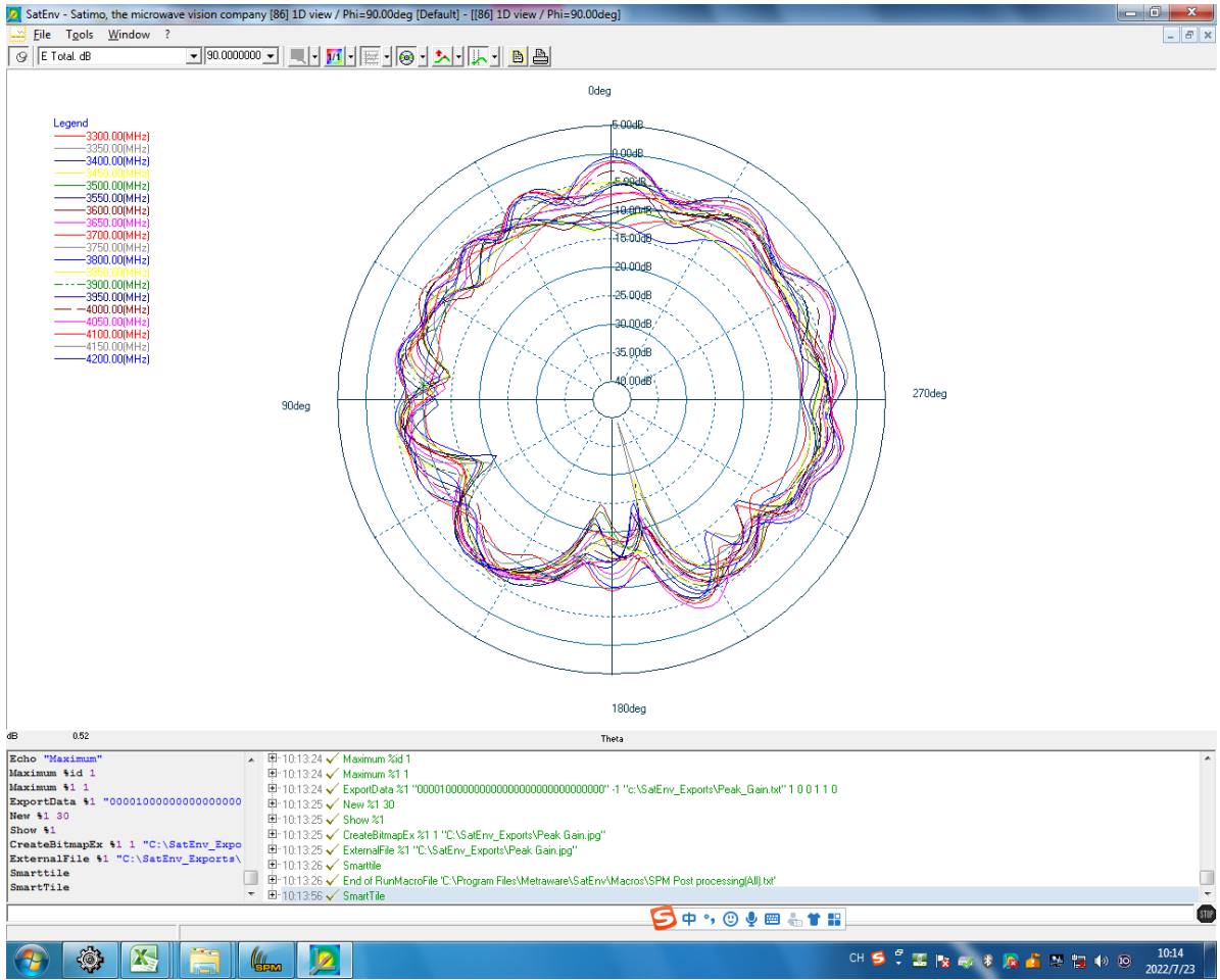
N77/N78 Phi=90deg
