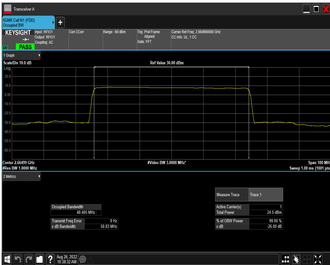
n41 SCS=15kHz DFT_QAM16 BW=50MHz Channel=532998 RB=270@0
