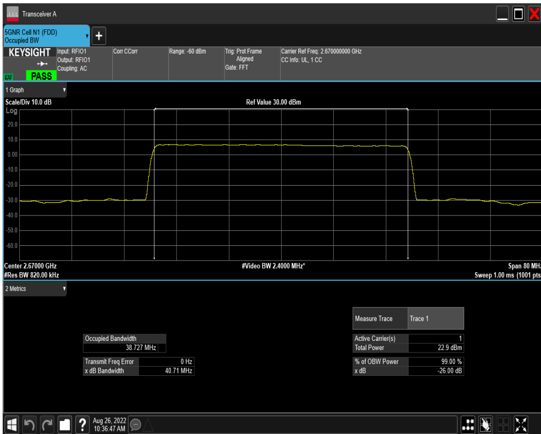
n41 SCS=15kHz DFT_QAM256 BW=40MHz Channel=534000 RB=216@0
