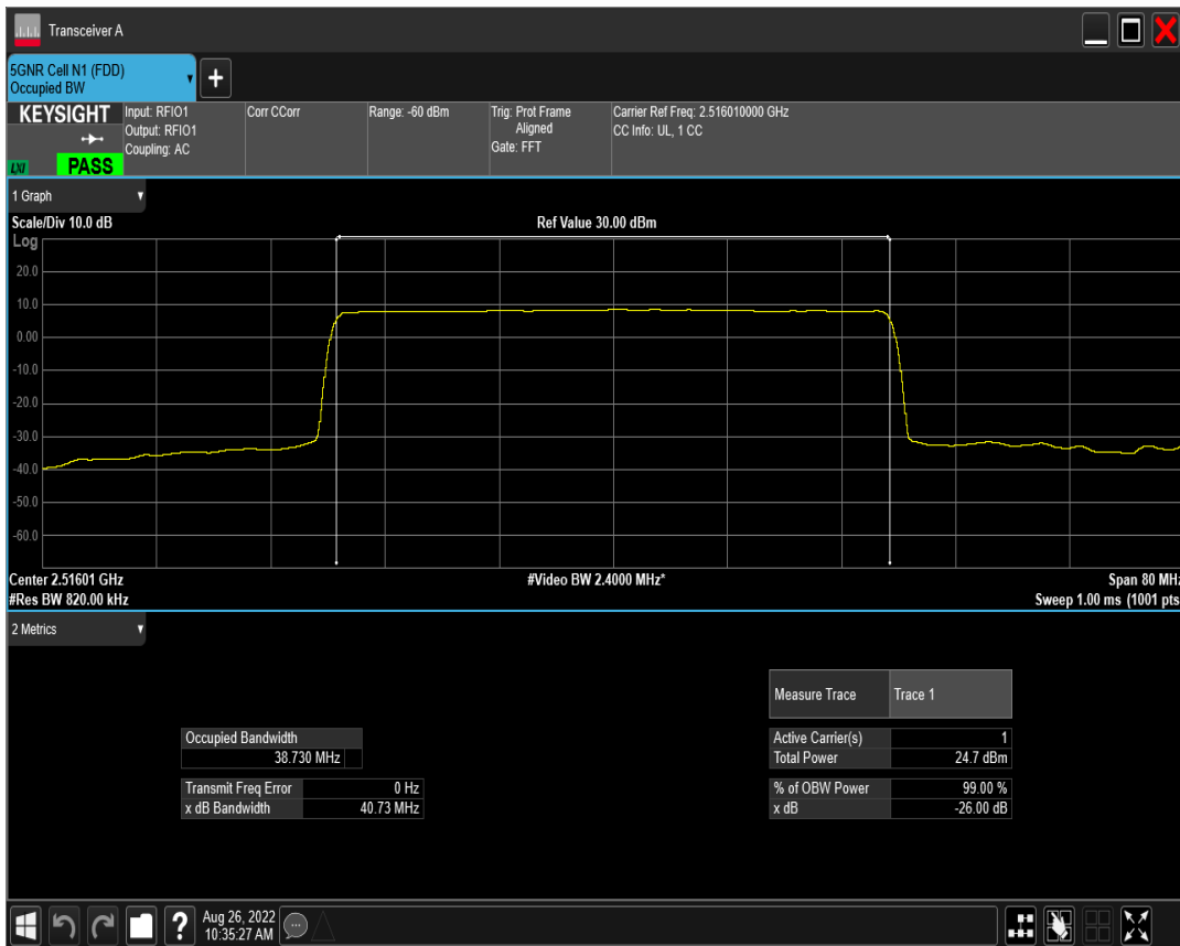
n41 SCS=15kHz DFT_QAM16 BW=40MHz Channel=503202 RB=216@0
