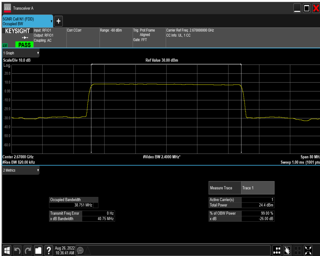
n41 SCS=15kHz DFT_QAM16 BW=40MHz Channel=534000 RB=216@0
