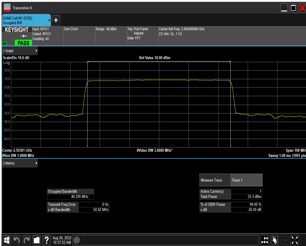
n41 SCS=15kHz DFT_QPSK BW=50MHz Channel=518601 RB=270@0
