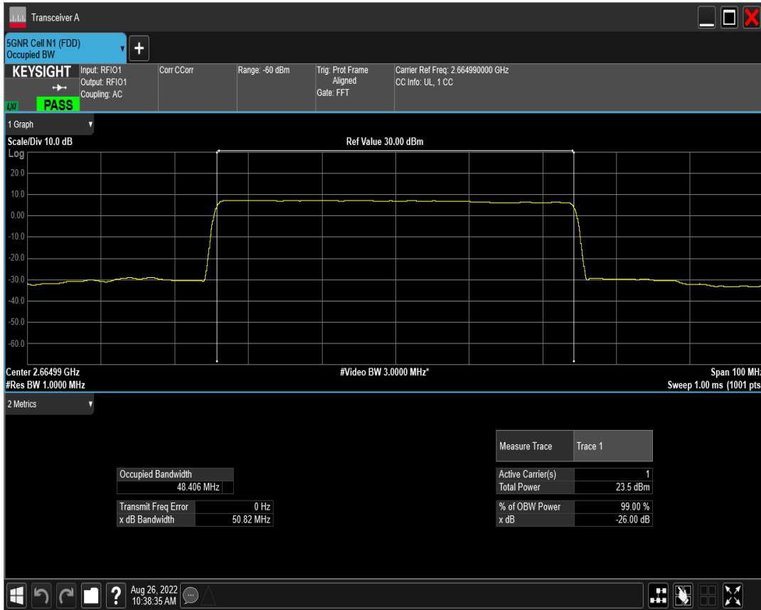
n41 SCS=15kHz DFT_QAM64 BW=50MHz Channel=532998 RB=270@0
