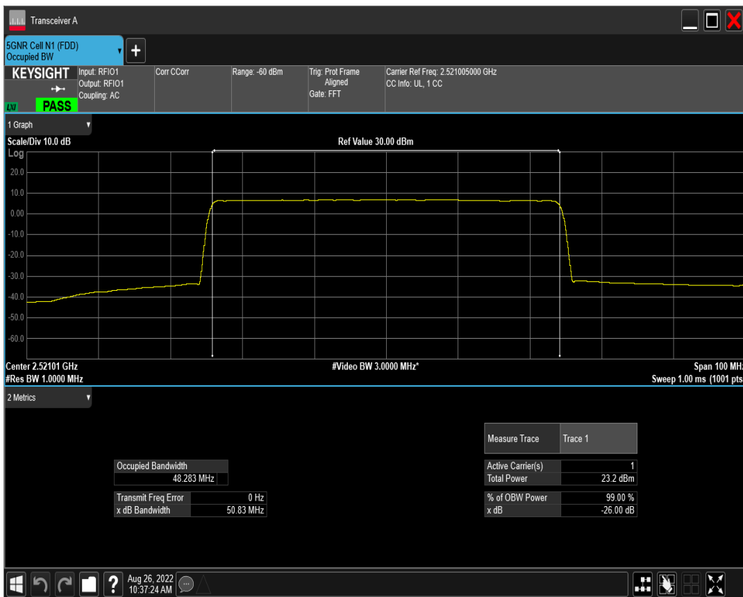
n41 SCS=15kHz DFT_QAM256 BW=50MHz Channel=504201 RB=270@0
