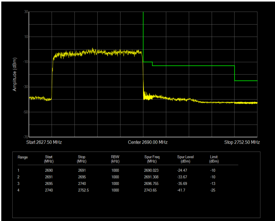
n41 SCS=15kHz DFT_QPSK BW=50MHz Channel=532998 RB=1@269
