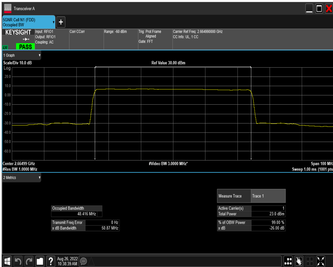
n41 SCS=15kHz DFT_QAM256 BW=50MHz Channel=532998 RB=270@0
