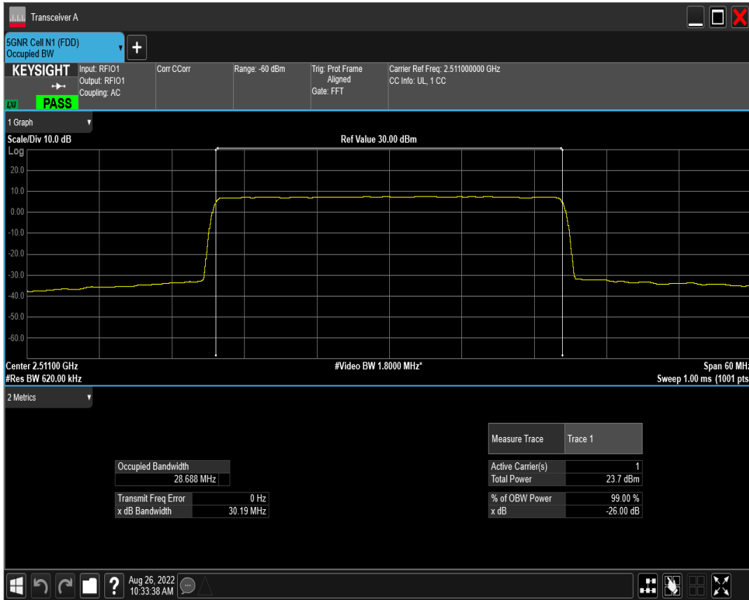
n41 SCS=15kHz DFT_QAM64 BW=30MHz Channel=502200 RB=160@0
