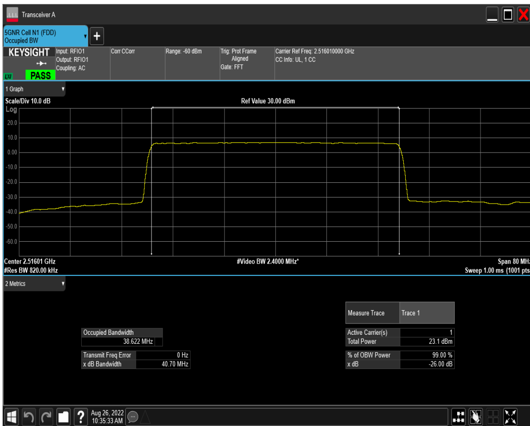
n41 SCS=15kHz DFT_QAM256 BW=40MHz Channel=503202 RB=216@0
