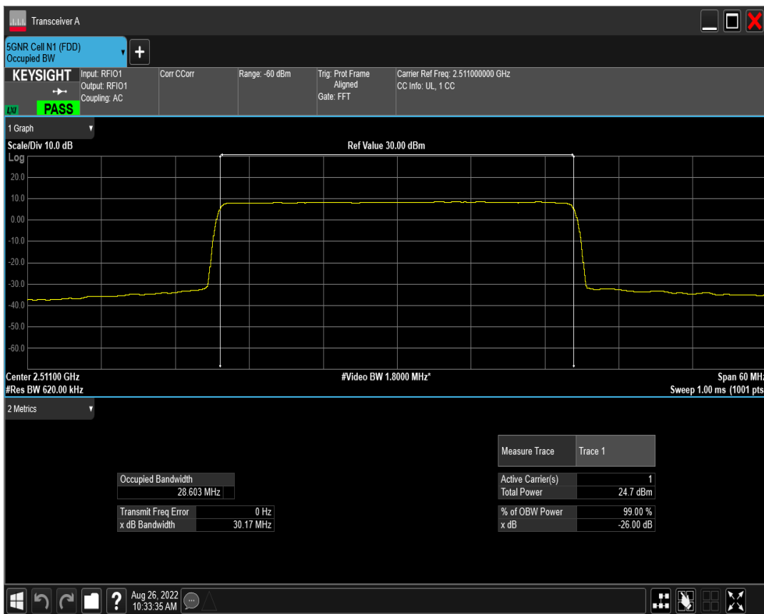
n41 SCS=15kHz DFT_QAM16 BW=30MHz Channel=502200 RB=160@0
