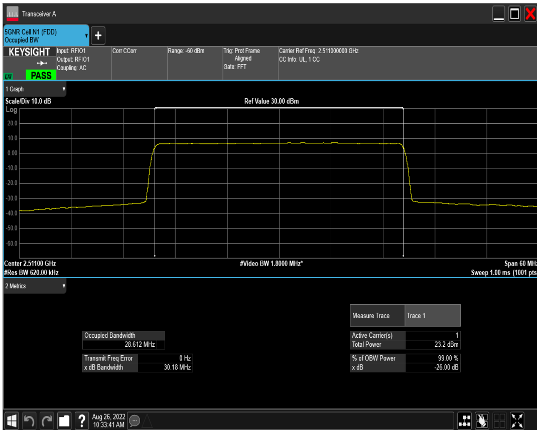
n41 SCS=15kHz DFT_QAM256 BW=30MHz Channel=502200 RB=160@0
