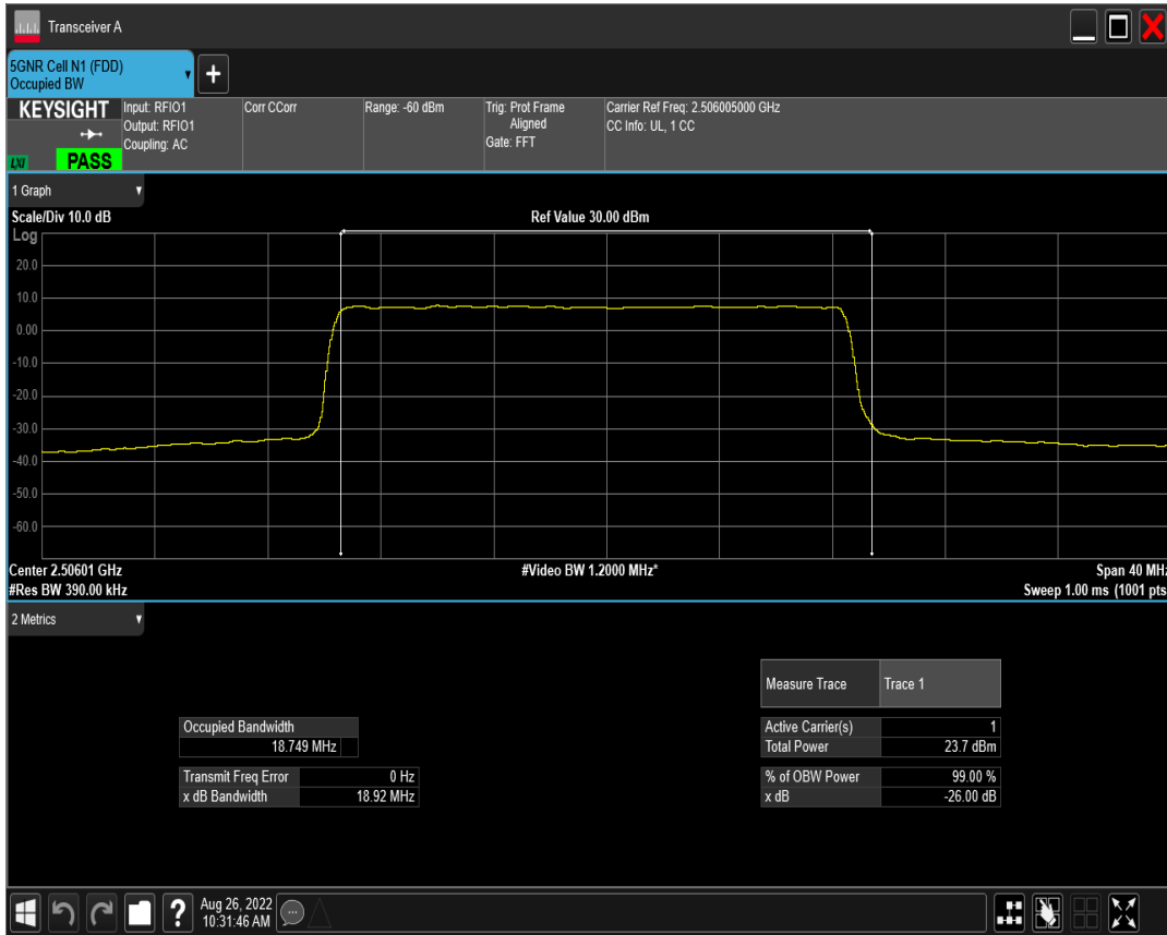
n41 SCS=15kHz DFT_QAM64 BW=20MHz Channel=501201 RB=100@0
