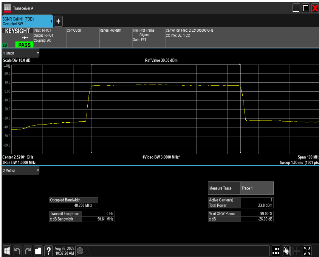
n41 SCS=15kHz DFT_QAM64 BW=50MHz Channel=504201 RB=270@0
