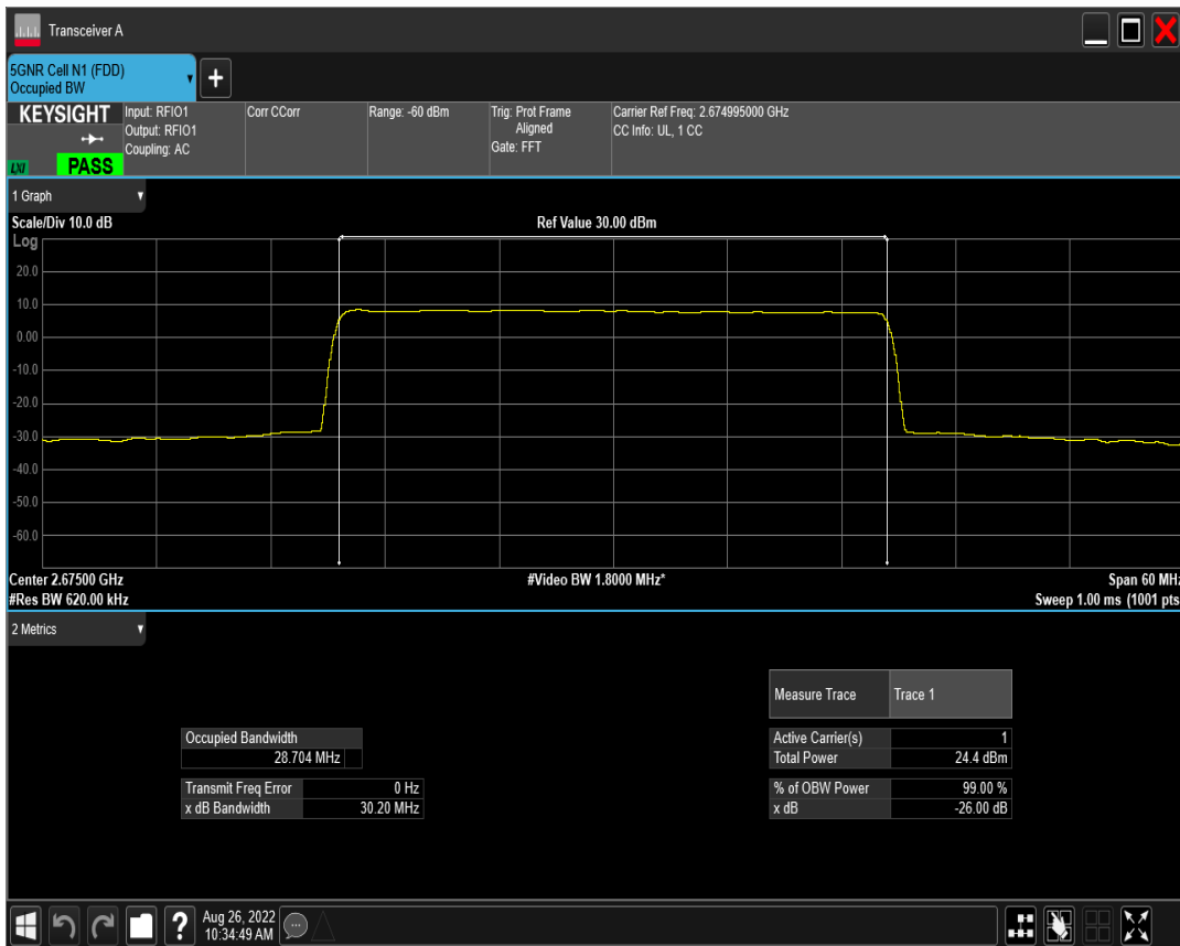
n41 SCS=15kHz DFT_QAM16 BW=30MHz Channel=534999 RB=160@0
