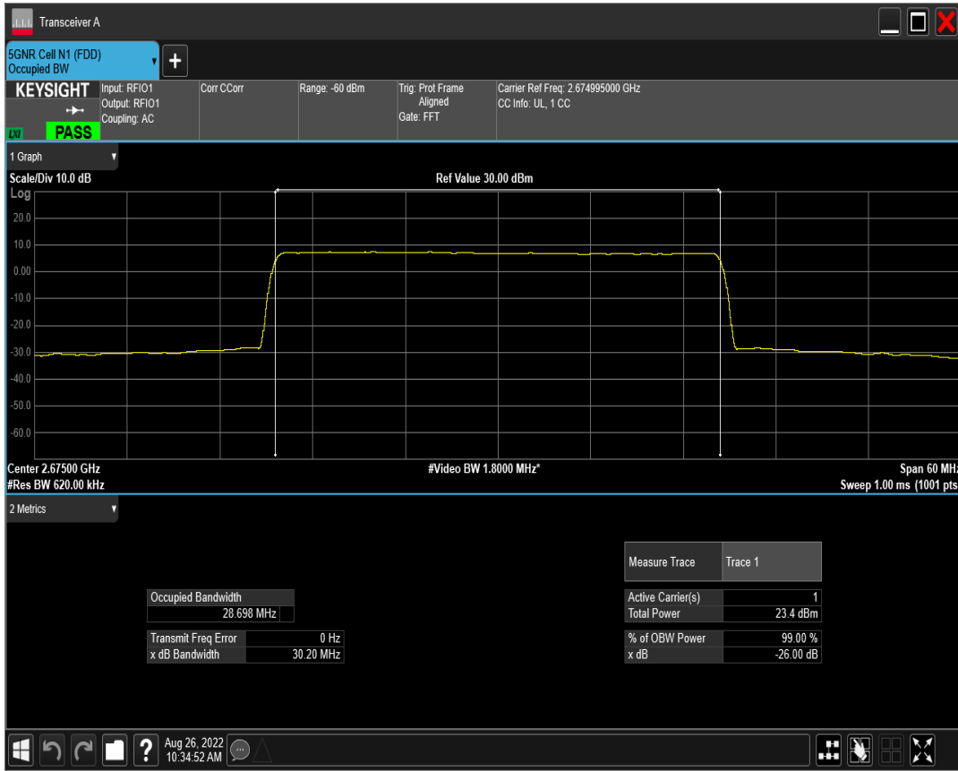
n41 SCS=15kHz DFT_QAM64 BW=30MHz Channel=534999 RB=160@0
