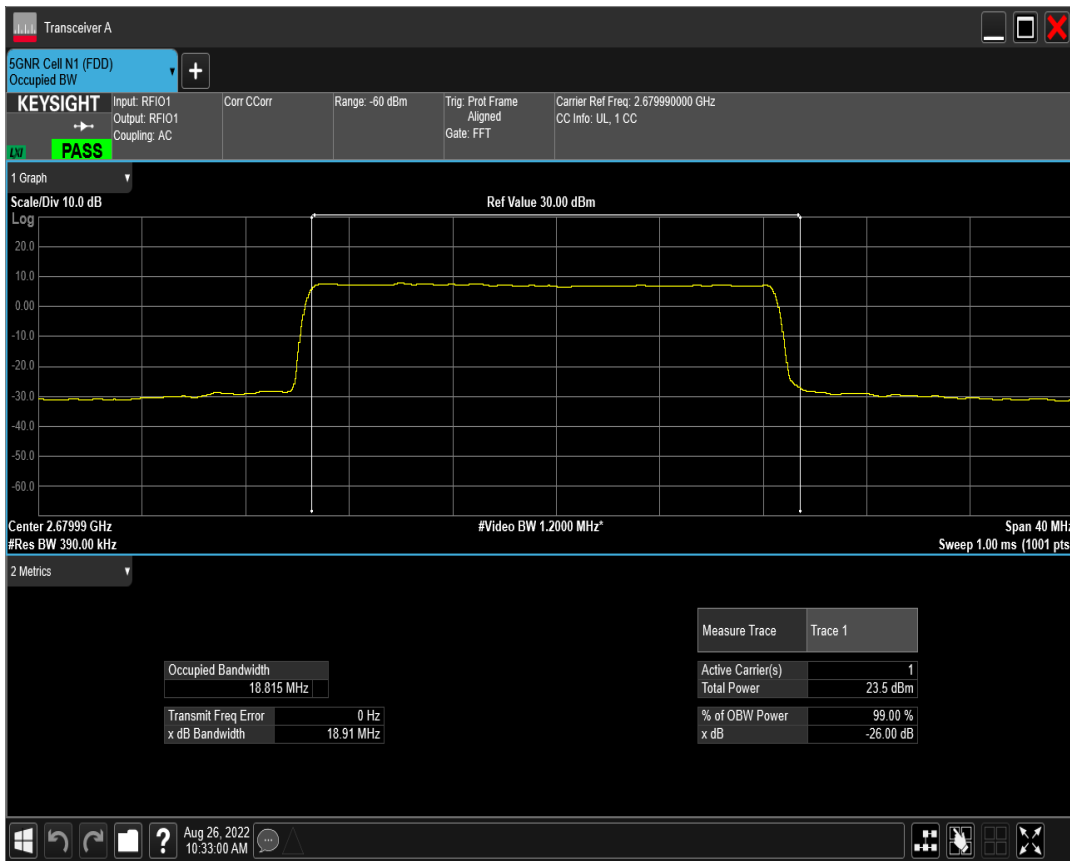
n41 SCS=15kHz DFT_QAM64 BW=20MHz Channel=535998 RB=100@0
