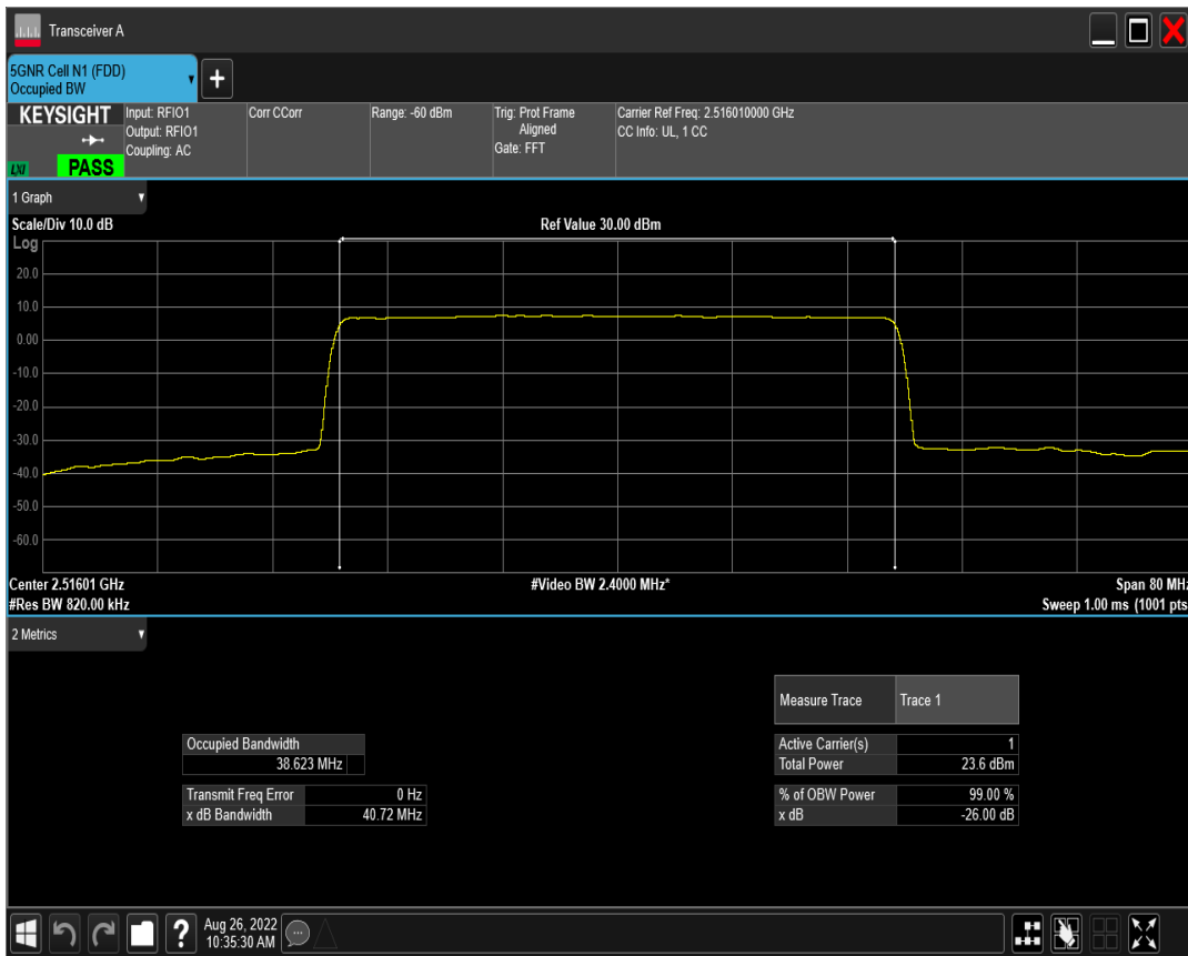
n41 SCS=15kHz DFT_QAM64 BW=40MHz Channel=503202 RB=216@0
