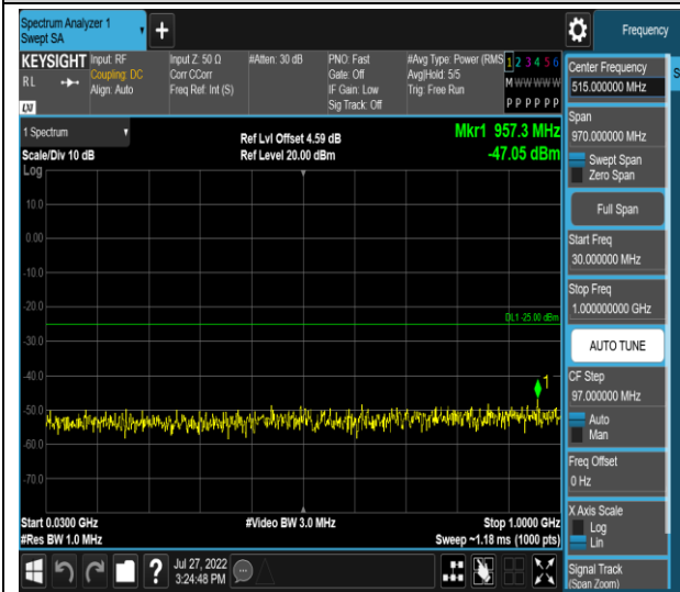
Band41-5MHz-16QAM-39675-1RB#0-Range1:30~1000MHz
