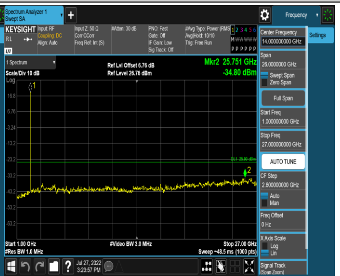
Band41-5MHz-16QAM-39675-1RB#0-Range2:1000~27000MHz
