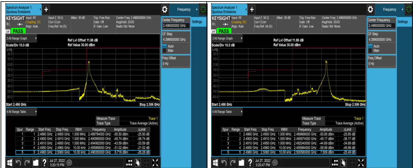
Band41-5MHz-16QAM-39675-25RB#0
