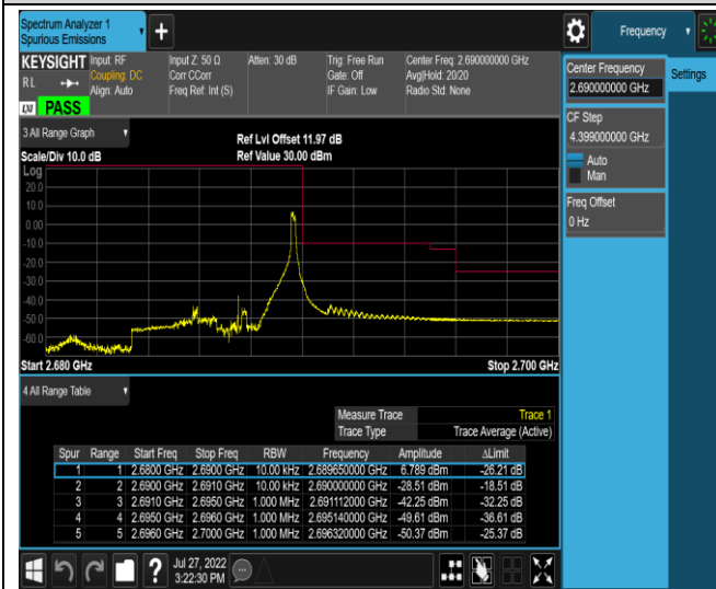
Band41-20MHz-QPSK-39750-1RB#0
