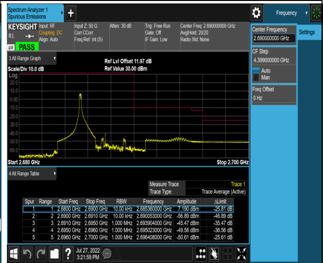
Band41-5MHz-16QAM-41565-25RB#0
