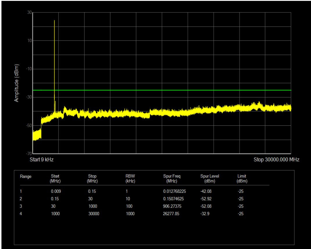
n41(2535-2655) SCS=15kHz DFT_QPSK BW=10MHz Channel=508002 RB=1 @51
