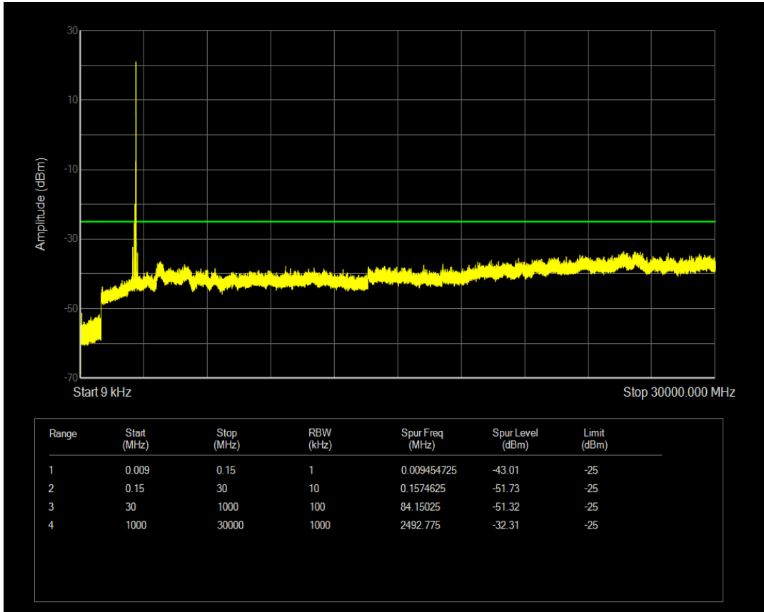
n41(2535-2655) SCS=15kHz DFT_QPSK BW=10MHz Channel=529998 RB=1@51
