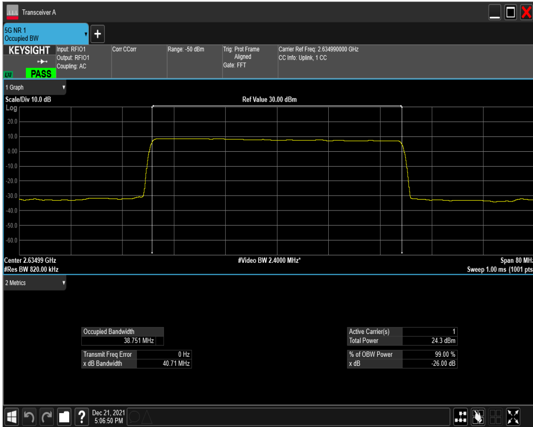
n41(2535-2655) SCS=15kHz DFT_QAM64 BW=40MHz Channel=526998 RB=216@0
