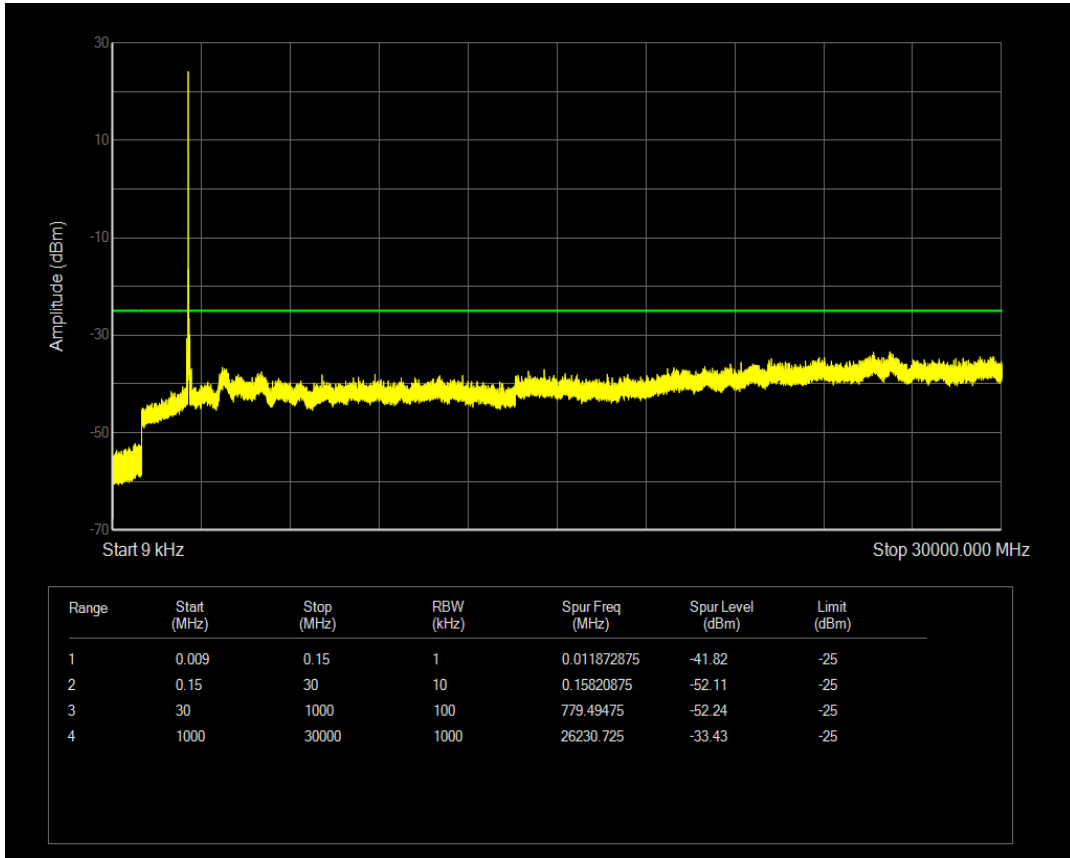
n41(2535-2655) SCS=15kHz DFT_QPSK BW=50MHz Channel=519000 RB=1@269
