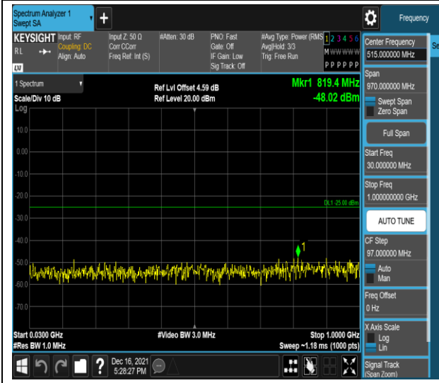
Band41-5MHz-16QAM-40640-1RB#0-Range1:30~1000MHz
