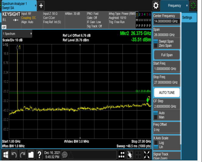
Band41-20MHz-16QAM-40140-1RB#0-Range2:1000~27000MHz
