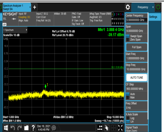
Band17-10MHz-16QAM-23800-1RB#0-Range2:1000~ 10000MHz
