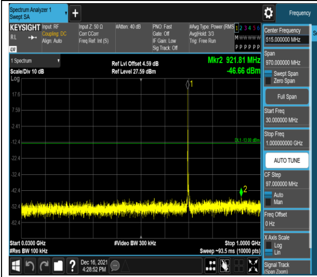
Band17-5MHz-QPSK-23790-1RB#0-Range1:30~1000MHz
