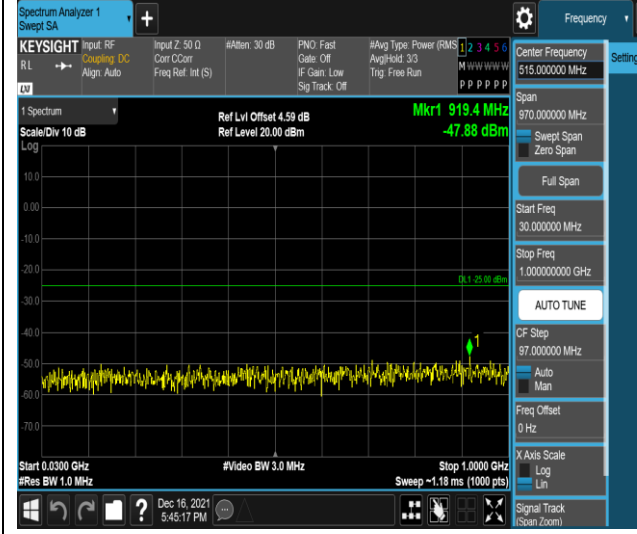
Band41-20MHz-16QAM-40140-1RB#0-Range1:30~1000MHz
