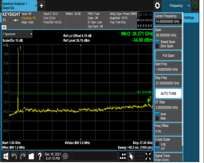
Band41-20MHz-16QAM-40140-1RB#0-Range2:1000~27000MHz
