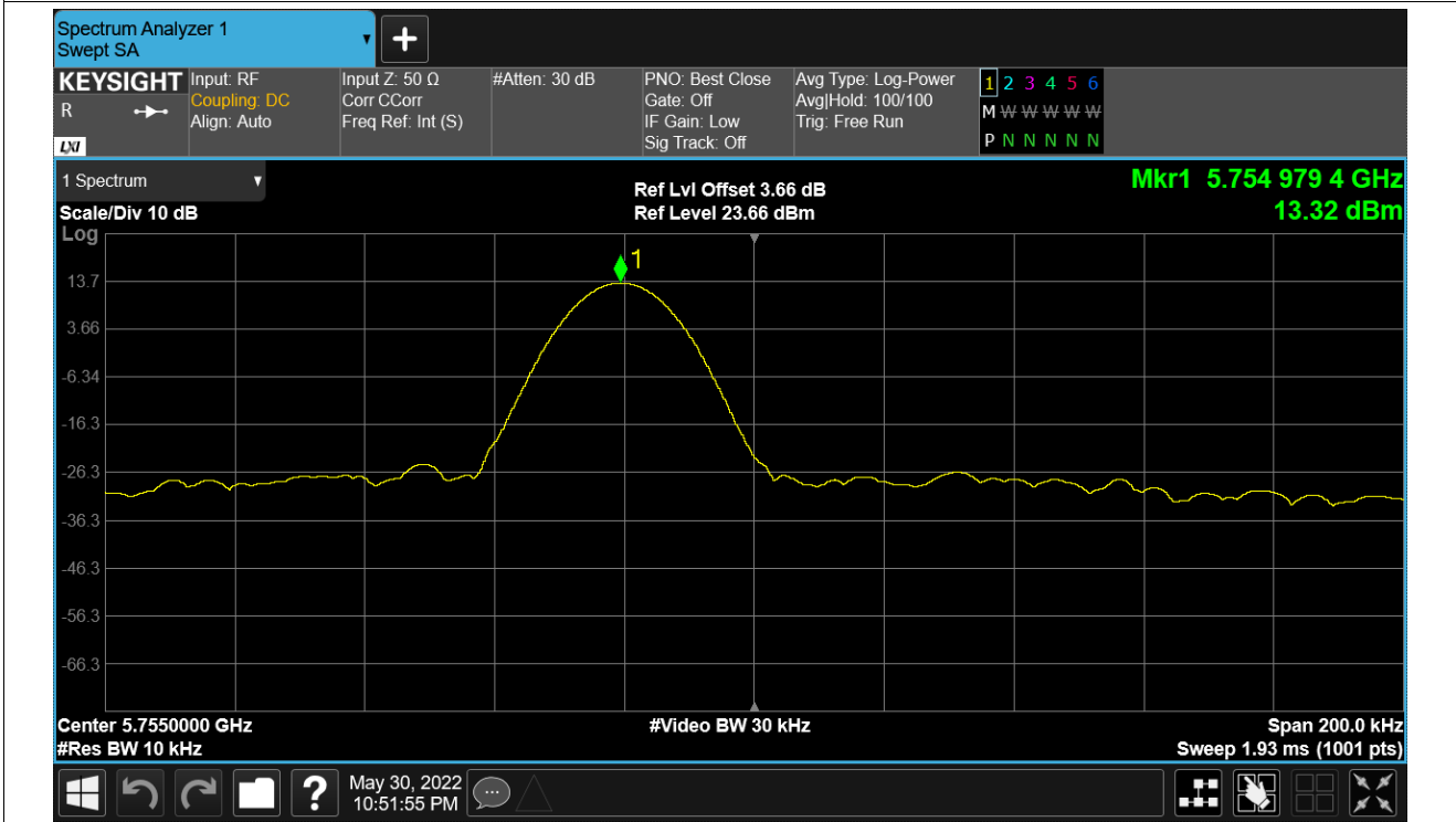
Freq. Stability NVNT n40 5755MHz Ant1
