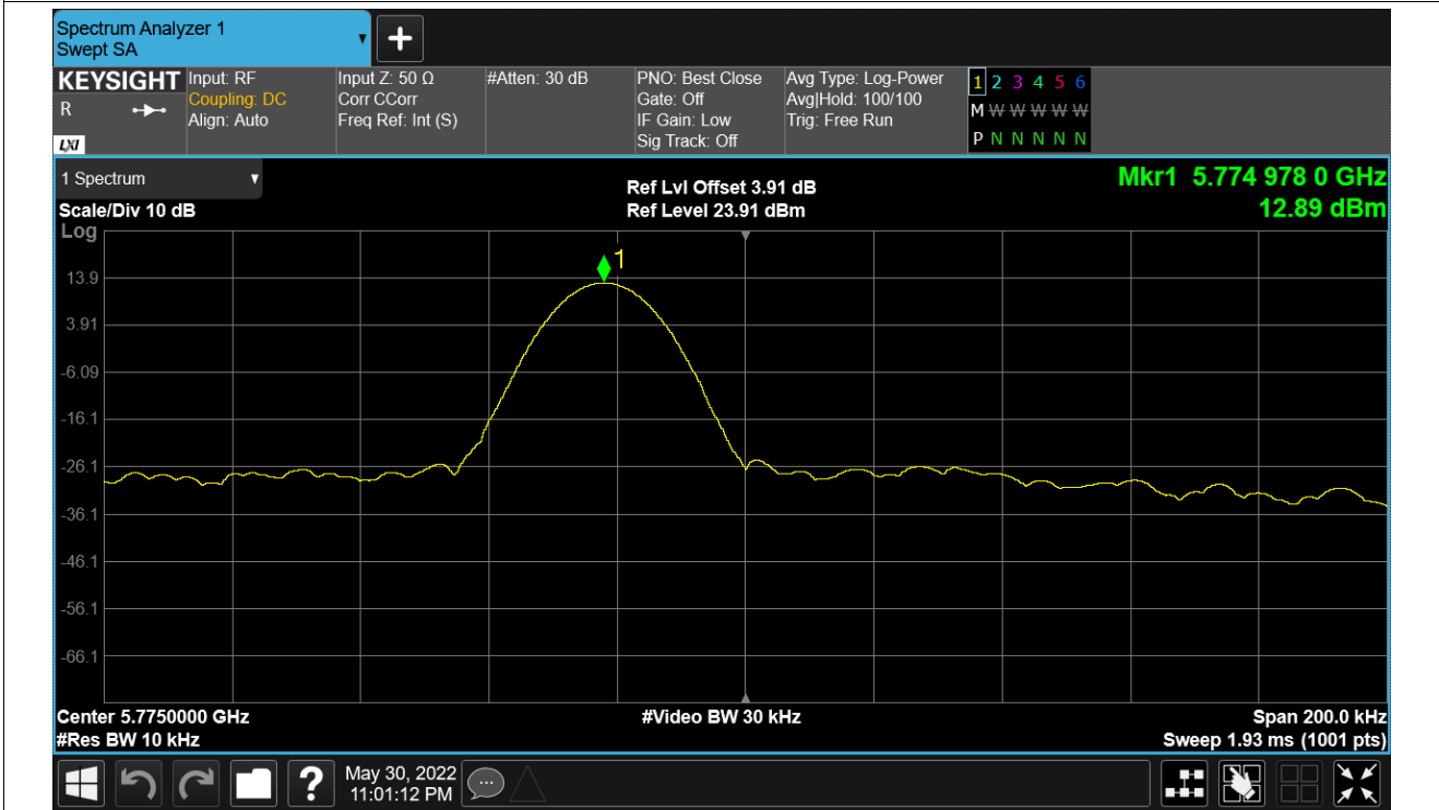
Freq. Stability LVNT ac80 5775MHz Ant1
