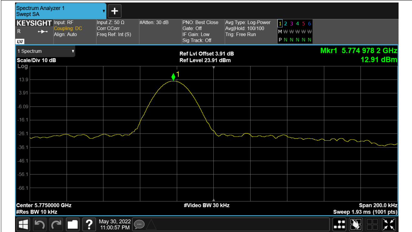
Freq. Stability NVLT ac80 5775MHz Ant1
