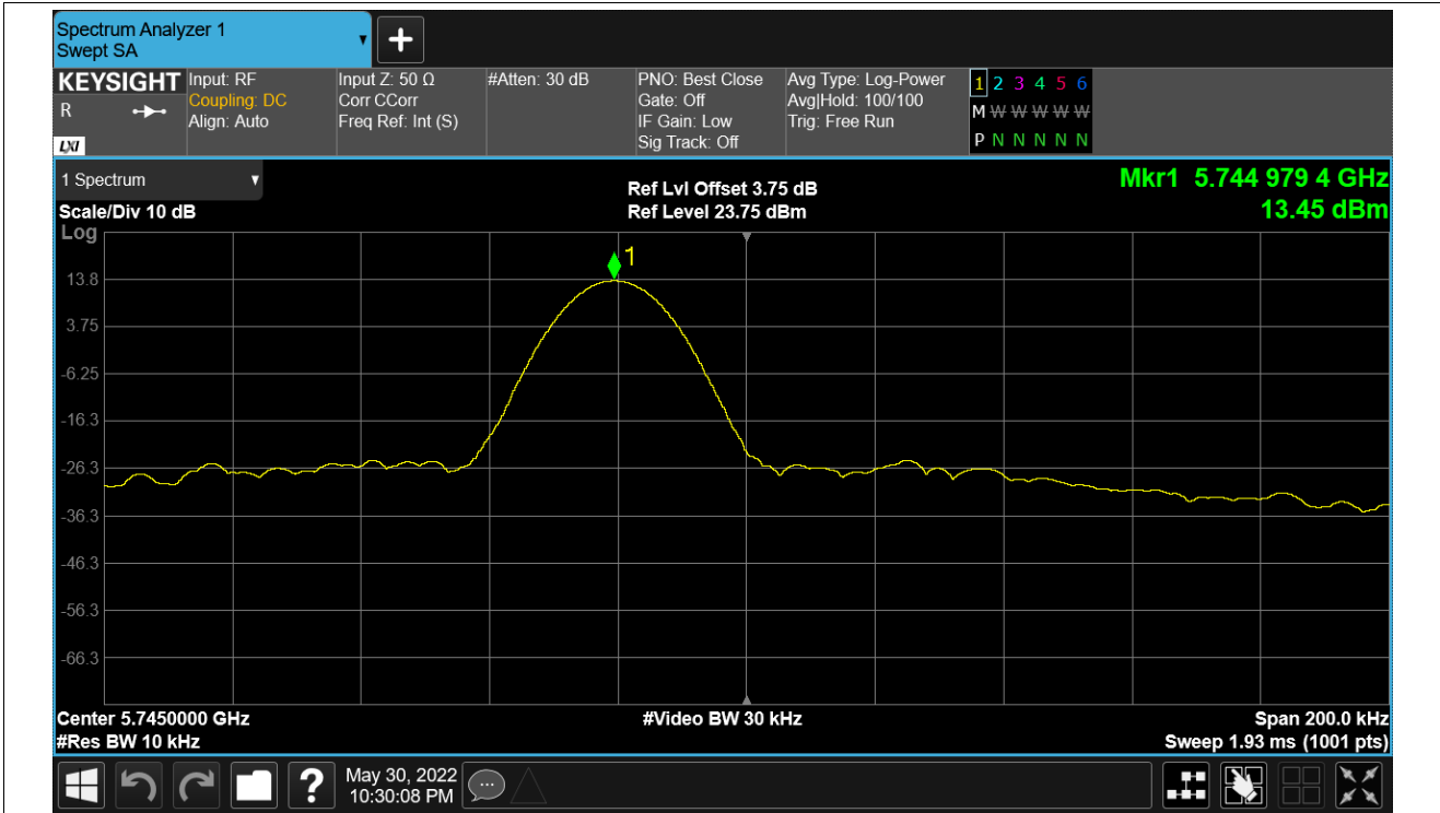
Freq. Stability NVLT a 5745MHz Ant1
