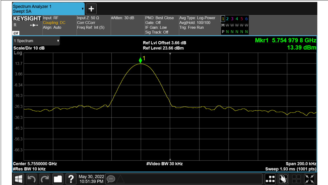
Freq. Stability NVHT n40 5755MHz Ant1
