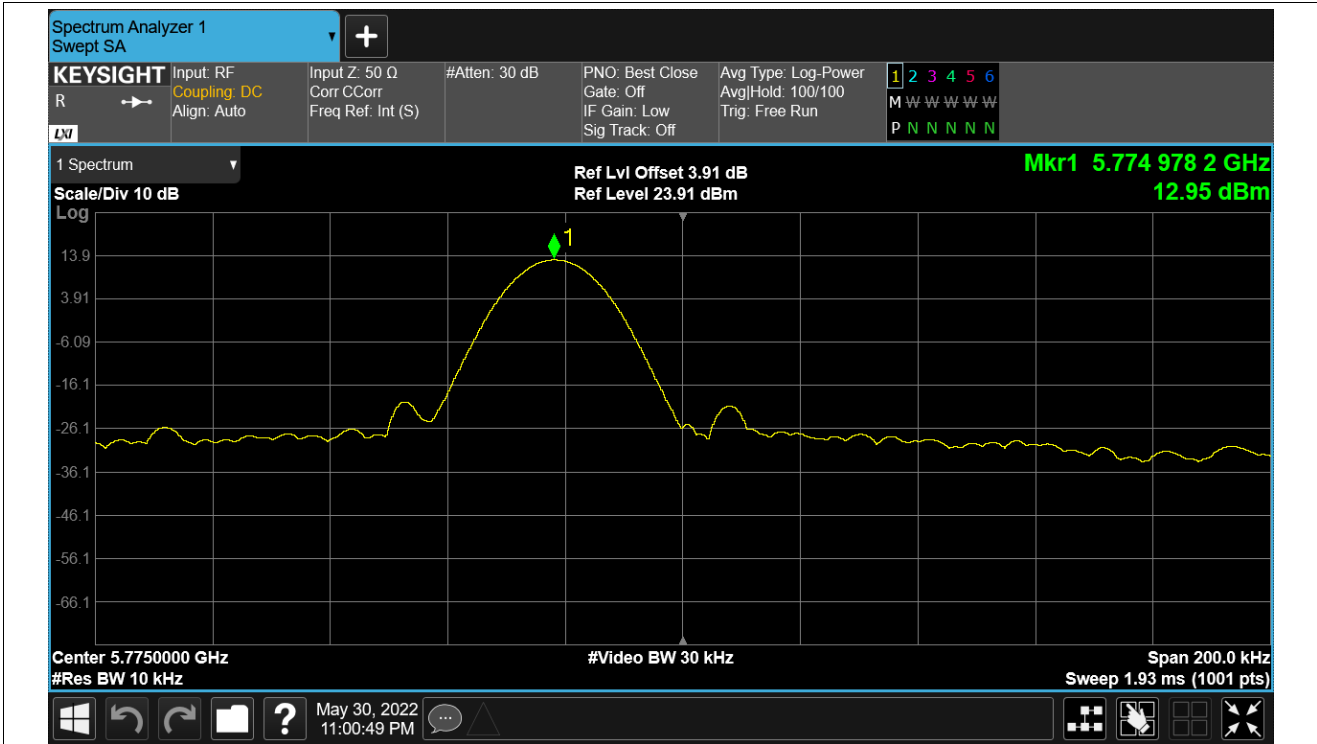
Freq. Stability NVNT ac80 5775MHz Ant1
