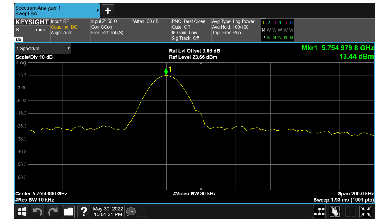
Freq. Stability NVLT n40 5755MHz Ant1
