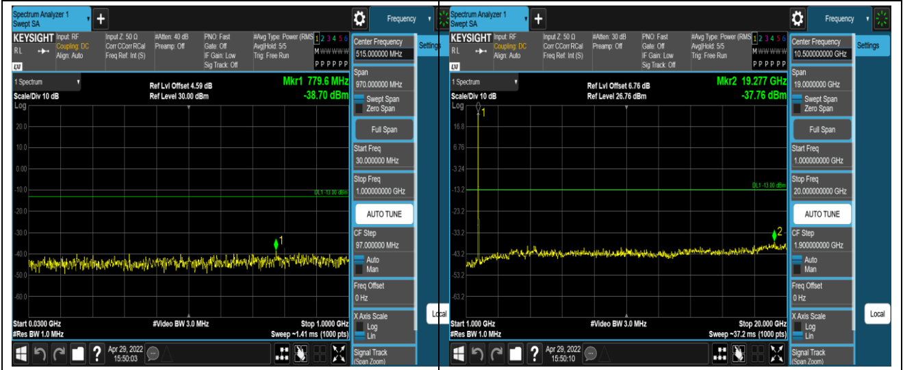
Band4-20MHz-QPSK-20300-1RB#0-Range1:30~1000MHz
