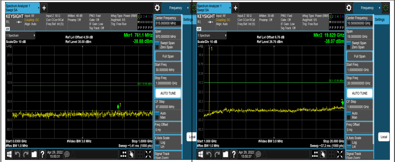
Band4-20MHz-16QAM-20050-1RB#0-Range1:30~1000MHz
