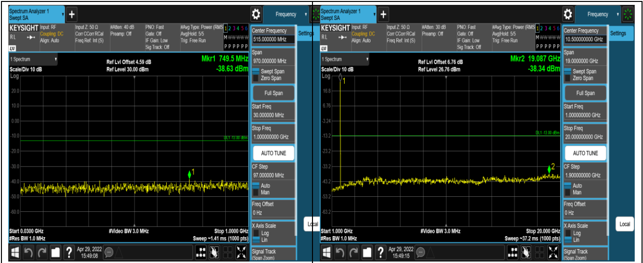
Band4-20MHz-QPSK-20175-1RB#0-Range1:30~1000MHz
