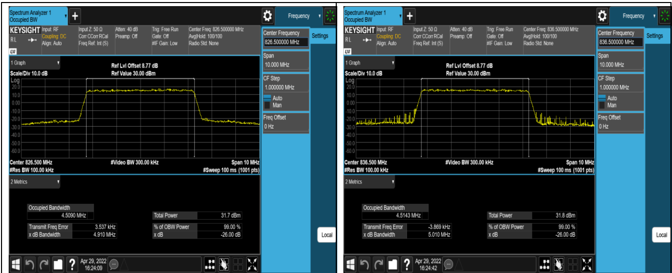
Band5-5MHz-QPSK-20625-25RB#0
