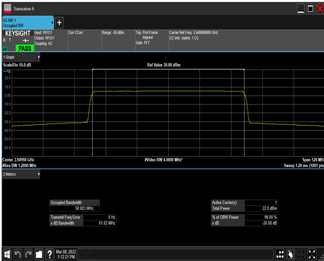
n77(3700-3980) SCS=30kHz CP_QPSK BW=60MHz Channel=663332 RB=162@0
