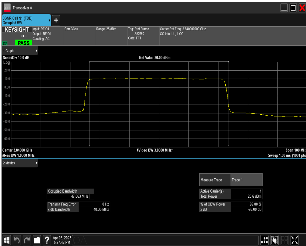
n77(3700-3980) SCS=30kHz DFT_QAM16 BW=50MHz Channel=656000 RB=128@0
