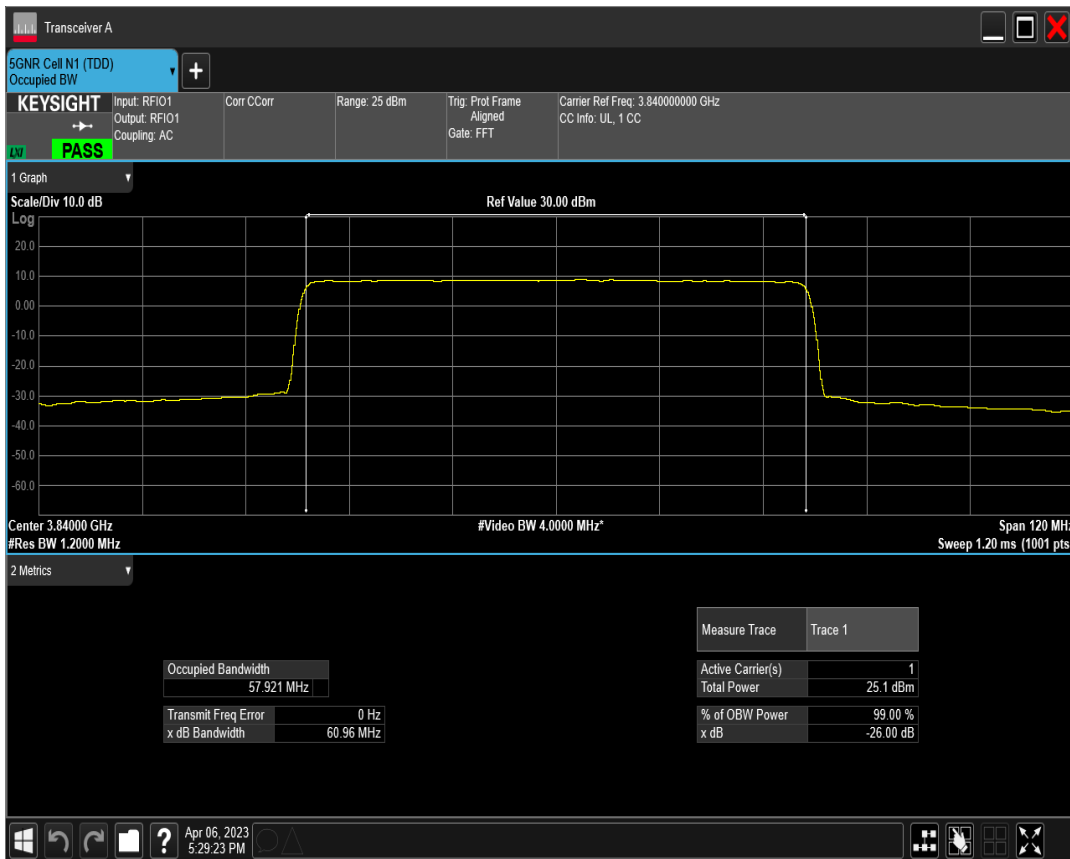
n77(3700-3980) SCS=30kHz DFT_QAM256 BW=60MHz Channel=656000 RB=162@0
