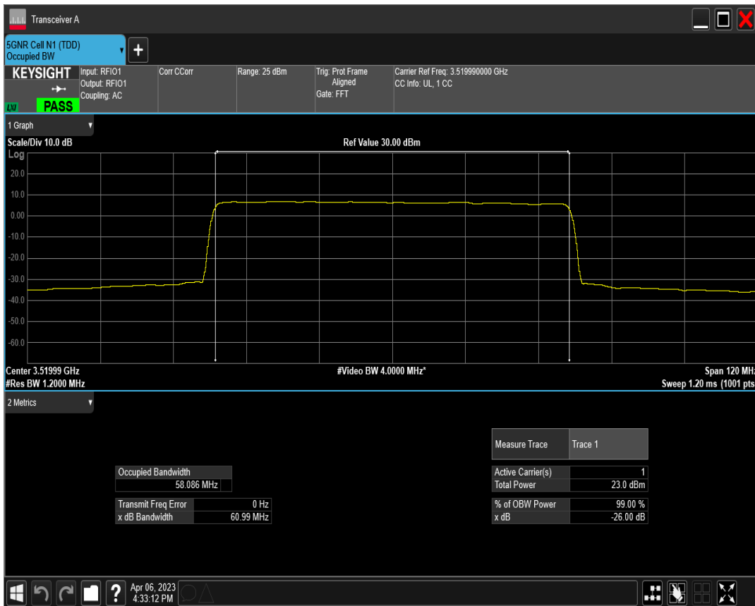
n77(3450-3550) SCS=30kHz CP_QPSK BW=60MHz Channel=634666 RB=162@0
