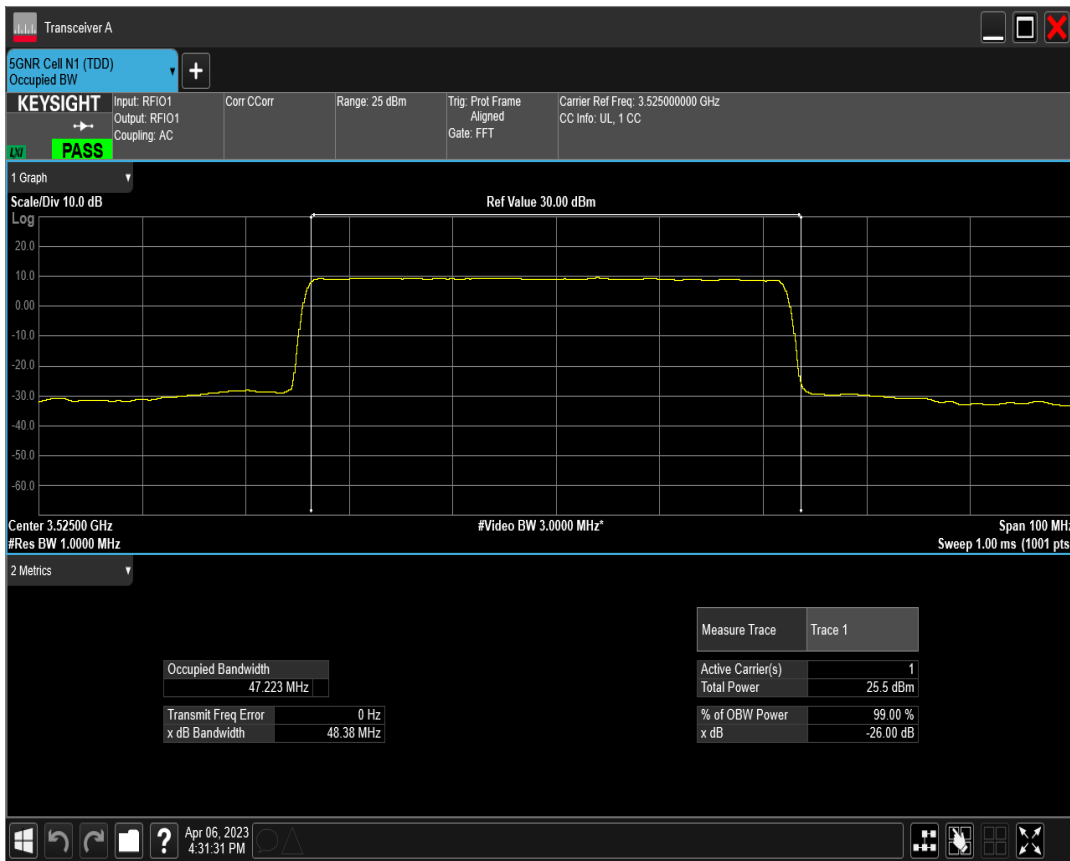
n77(3450-3550) SCS=30kHz DFT_QAM64 BW=50MHz Channel=635000 RB=128@0
