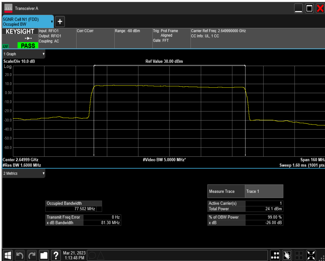
n41 SCS=30kHz DFT_QAM64 BW=80MHz Channel=52998 RB=216@0
