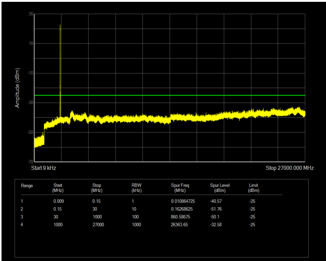
n38 SCS=15kHz DFT_QPSK BW=5MHz Channel=518500 RB=1@0
