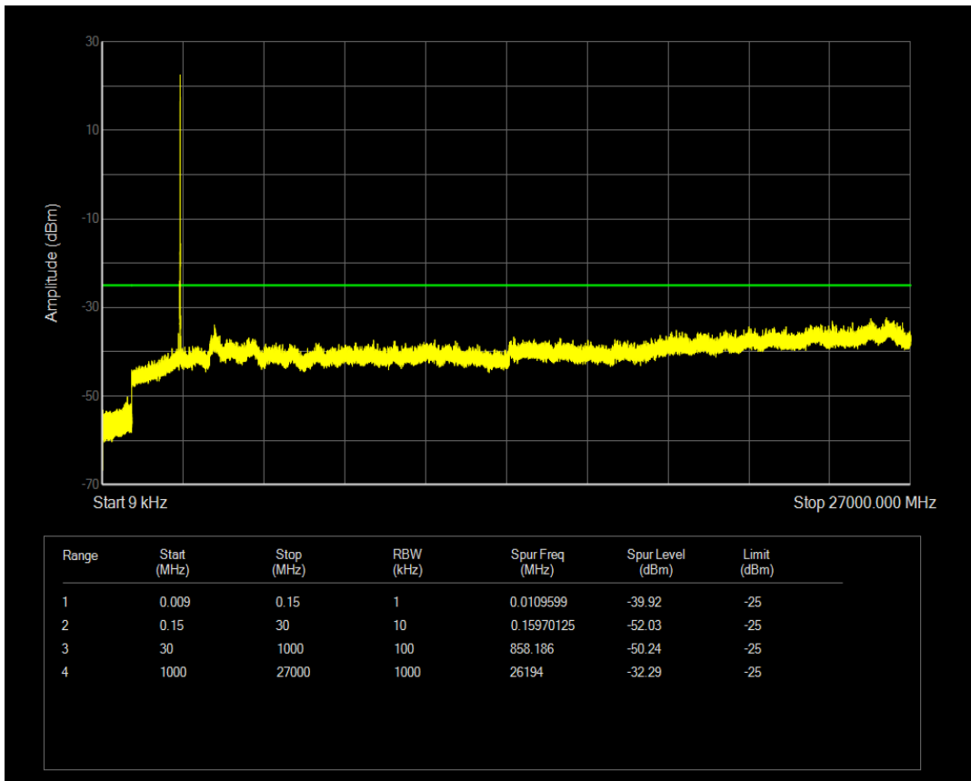
n38 SCS=15kHz DFT_QPSK BW=5MHz Channel=523500 RB=1@0
