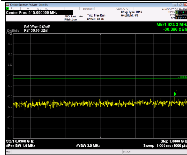
Band66-1.4MHz-64QAM-131979-1RB#0-Range1:3 0~1000MHz
