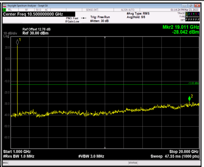
Band66-1.4MHz-64QAM-131979-1RB#0-Range2:100 0~20000MHz
