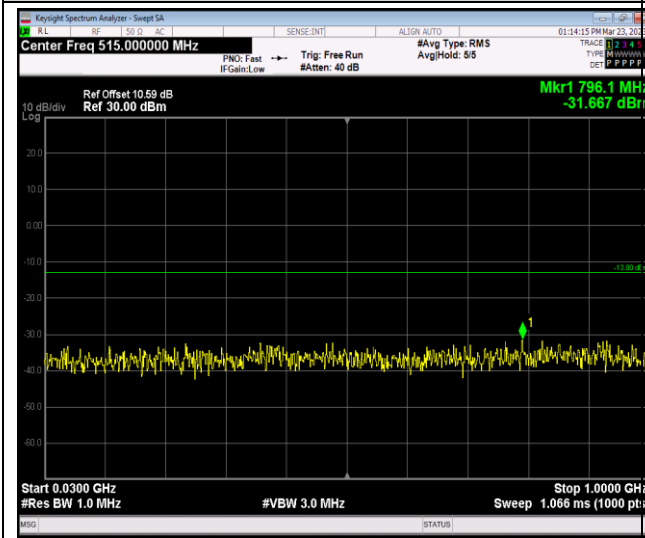
Band66-1.4MHz-64QAM-131979-1RB#0-Range1:3 0~1000MHz
