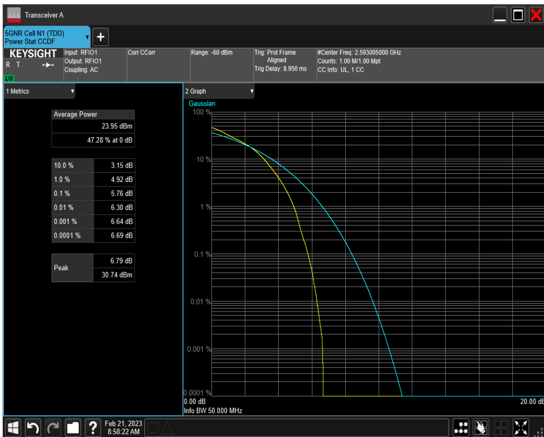
n41 SCS=15kHz DFT_QAM64 BW=50MHz Channel=518601 RB=270@0
