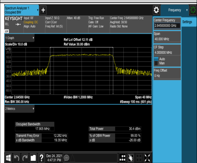
Band41-20MHz-16QAM-41140-100RB#0
