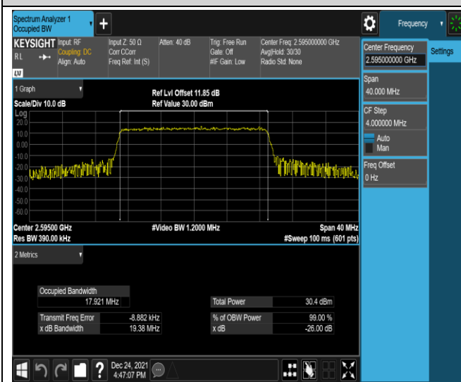
Band41-20MHz-16QAM-40640-100RB#0
