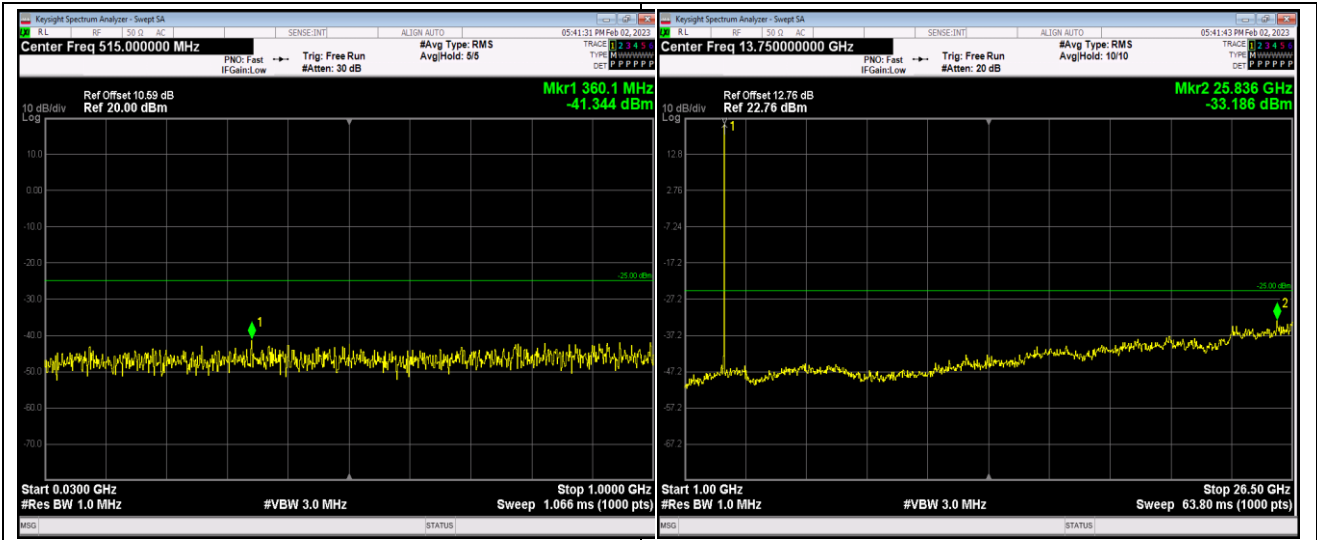
Band41-5MHz-64QAM-40065-1RB#0-Range1:30~1000MHz
