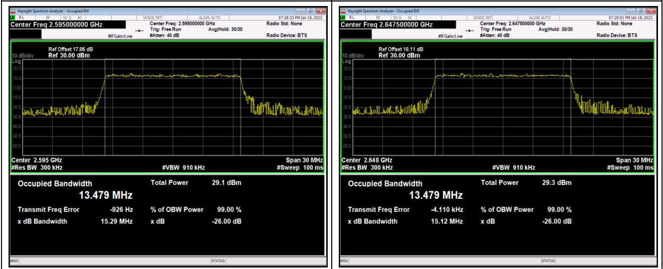
Band41-15MHz-64QAM-40115-75RB#0
