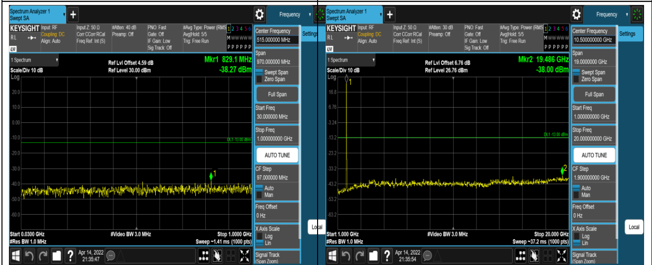
Band4-20MHz-QPSK-20300-1RB#0-Range1:30~1000MHz
