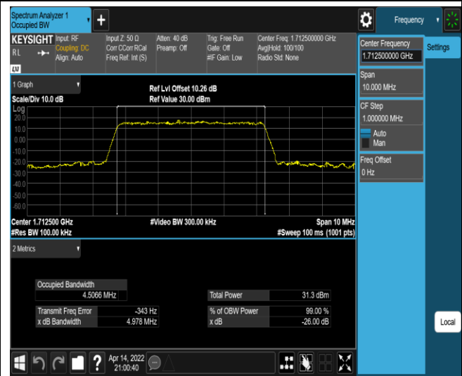
Band4-5MHz-16QAM-20375-25RB#0
