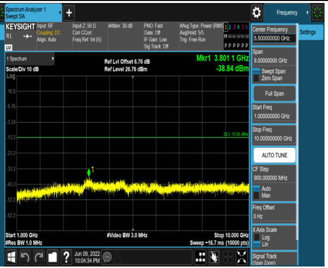
Band5-10MHz-16QAM-20600-1RB#0-Range2:1000~10000MHz
