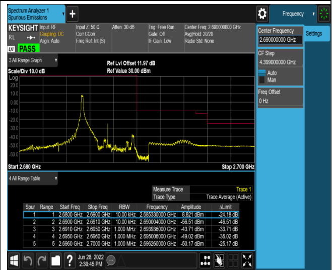
Band41-5MHz-QPSK-41565-25RB#0
