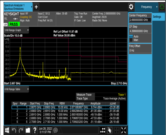
Band41-20MHz-QPSK-41490-100RB#0
