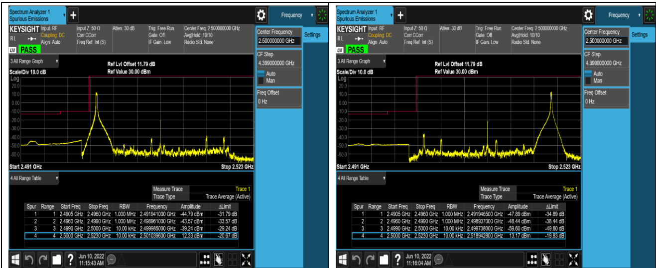
Band7-20MHz-QPSK-20850-100RB#0
