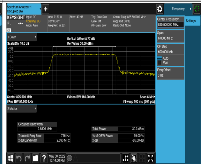
Band5-3MHz-16QAM-20635-15RB#0
