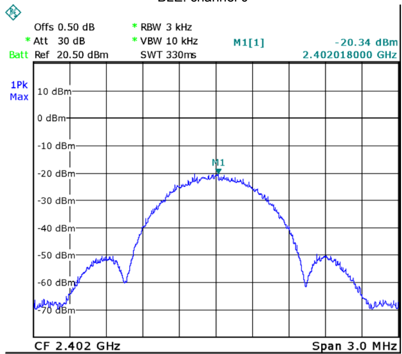
BLE: channel 0
