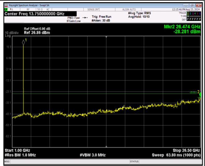
Band41-5MHz-64QAM-40640-1RB#0-Range2:1000~ 26500MHz
