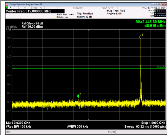
Band7-5MHz-QPSK-20775-1RB#0-Range1:30~1000 MHz
