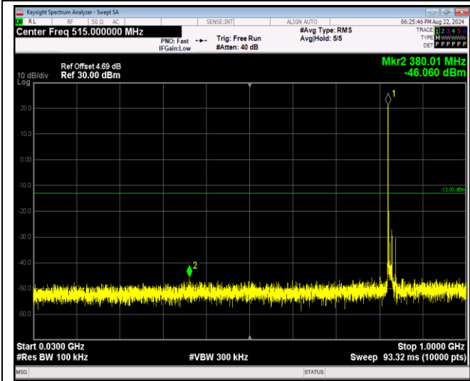
Band5-10MHz-16QAM-20525-1RB#0-Range1:30~100 OMHz
