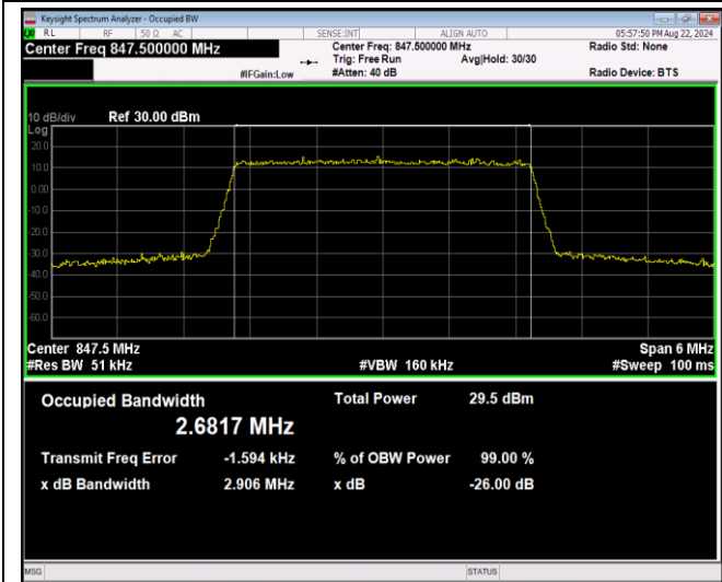
Band5-3MHz-64QAM-20525-15RB#0
