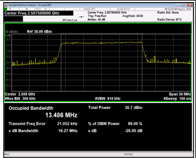
Band7-15MHz-16QAM-21375-75RB#0
